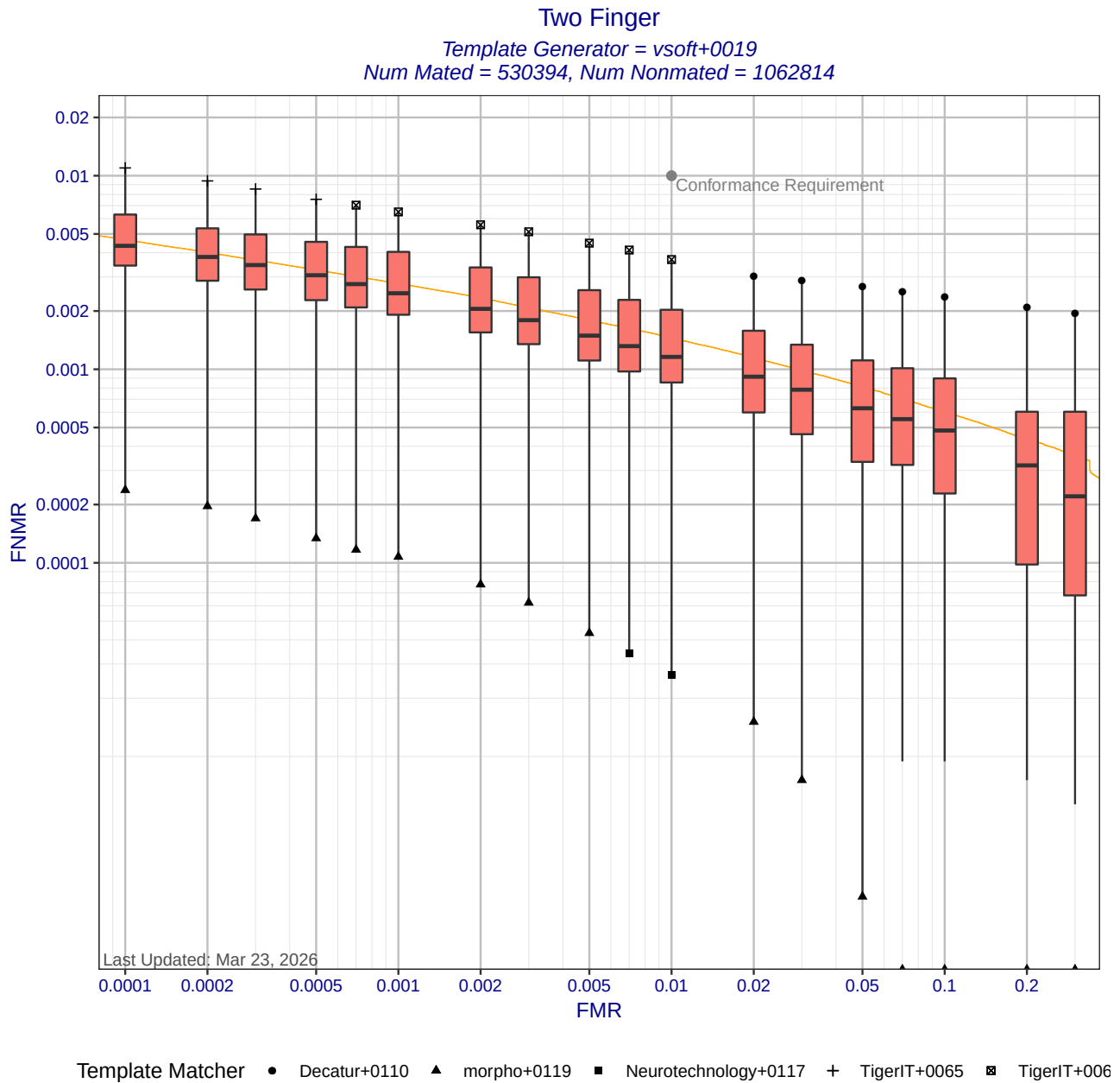
Figure 6: Two Finger DET statistics for template generator vsoft+0019. Each box shows the distribution of FNMNRs at a fixed FMR across different matchers. The whisker ends show the minimum and maximum FNMNRs. The orange DET curve shows pooled performance when all matchers use templates created by vsoft+0019. Score-level fusion is achieved by averaging the scores for left and right index fingers.
