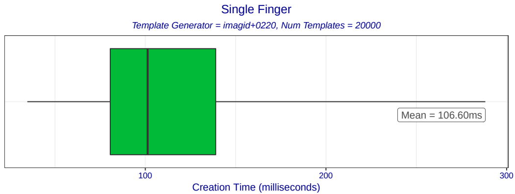
Figure 8: Boxplot of template creation times for template generator imagid+0220 . The box edges mark the 10th and 90th percentiles while the whiskers mark the maximum and minimum creation times.
