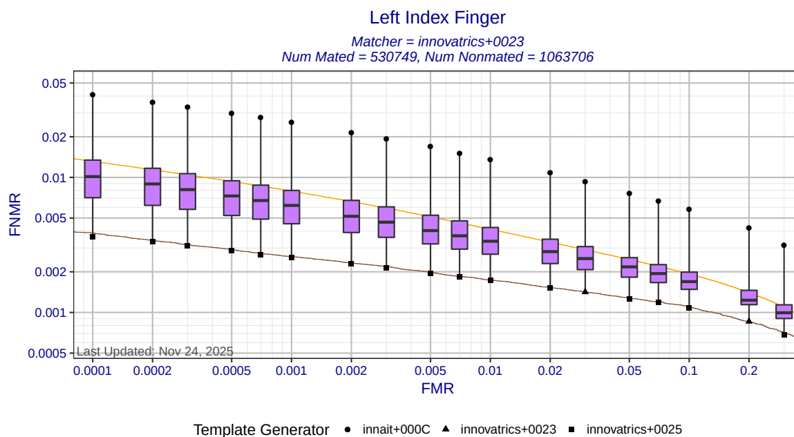
Figure 4: Left index finger DET statistics for matcher innovatrics+0023. Each box shows the distribution of FNMRs at a fixed FMR across all MINEX III compliant template generators. The ends of whiskers show the minimum and maximum FNMRs. The orange DET curve shows pooled performance against all template generators.
