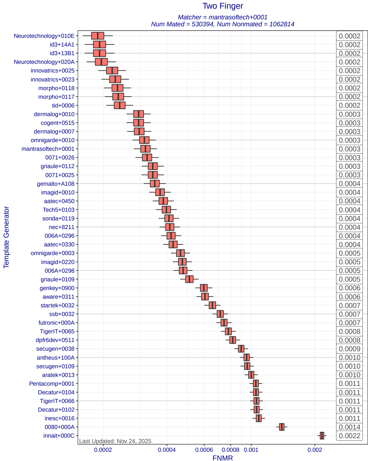
Figure 8: Two finger FNMR at FMR=0.01 when matcher mantrasoftech+0001 compares templates created by different template generators. Each box represents uncertainty about the true FNMR. The box edges mark the 50% confidence intervals while the whiskers mark the 90% confidence intervals. The numbers on the right show the actual computed FNMRs. Score-level fusion is achieved by averaging the scores for left and right index fingers.
