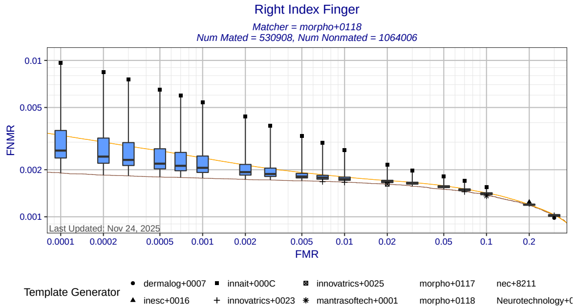
Figure 3: Right index finger DET statistics for matcher morpho+0118. Each box shows the distribution of FNMR at a fixed FMR across all MINEX III compliant template generators. The ends of the whiskers show the minimum and maximum FNMRs. The orange DET curve shows pooled performance against all template generators.
