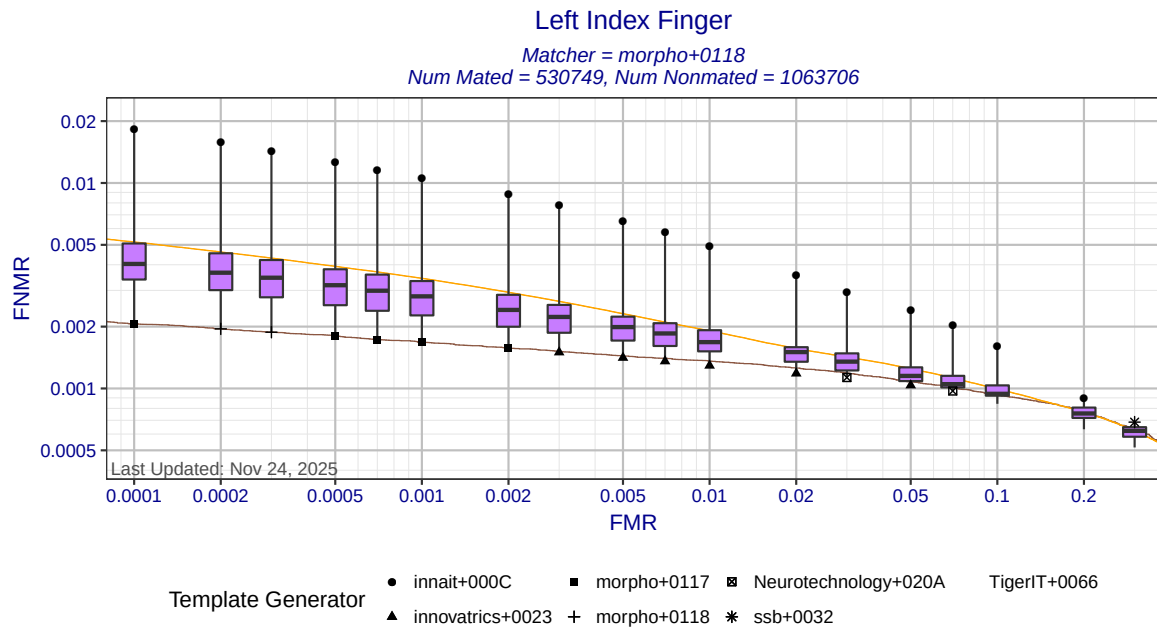
Figure 4: Left index finger DET statistics for matcher morpho+0118. Each box shows the distribution of FNMRs at a fixed FMR across all MINEX III compliant template generators. The ends of whiskers show the minimum and maximum FNMRs. The orange DET curve shows pooled performance against all template generators.
