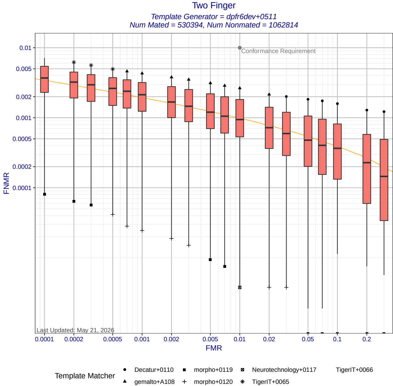
Figure 6: Two Finger DET statistics for template generator dpfr6dev+0511. Each box shows the distribution of FNRs at a fixed FMR across different matchers. The whisker ends show the minimum and maximum FNRs. The orange DET curve shows pooled performance when all matchers use templates created by dpfr6dev+0511. Score-level fusion is achieved by averaging the scores for left and right index fingers.
