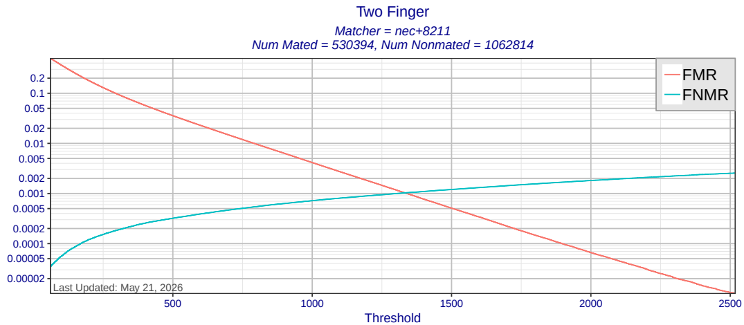
Figure 12: Two finger FMR and FNMR as a function of score threshold for matcher nec+8211 using templates created by all MINEX III compliant template generators. Score-level fusion is achieved by averaging scores for the left and right index fingers.
