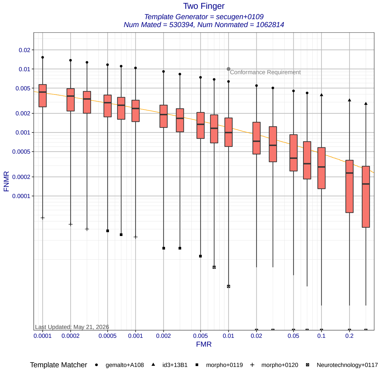
Figure 6: Two Finger DET statistics for template generator secugen+0109. Each box shows the distribution of FNMRs at a fixed FMR across different matchers. The whisker ends show the minimum and maximum FNMRs. The orange DET curve shows pooled performance when all matchers use templates created by secugen+0109. Score-level fusion is achieved by averaging the scores for left and right index fingers.
