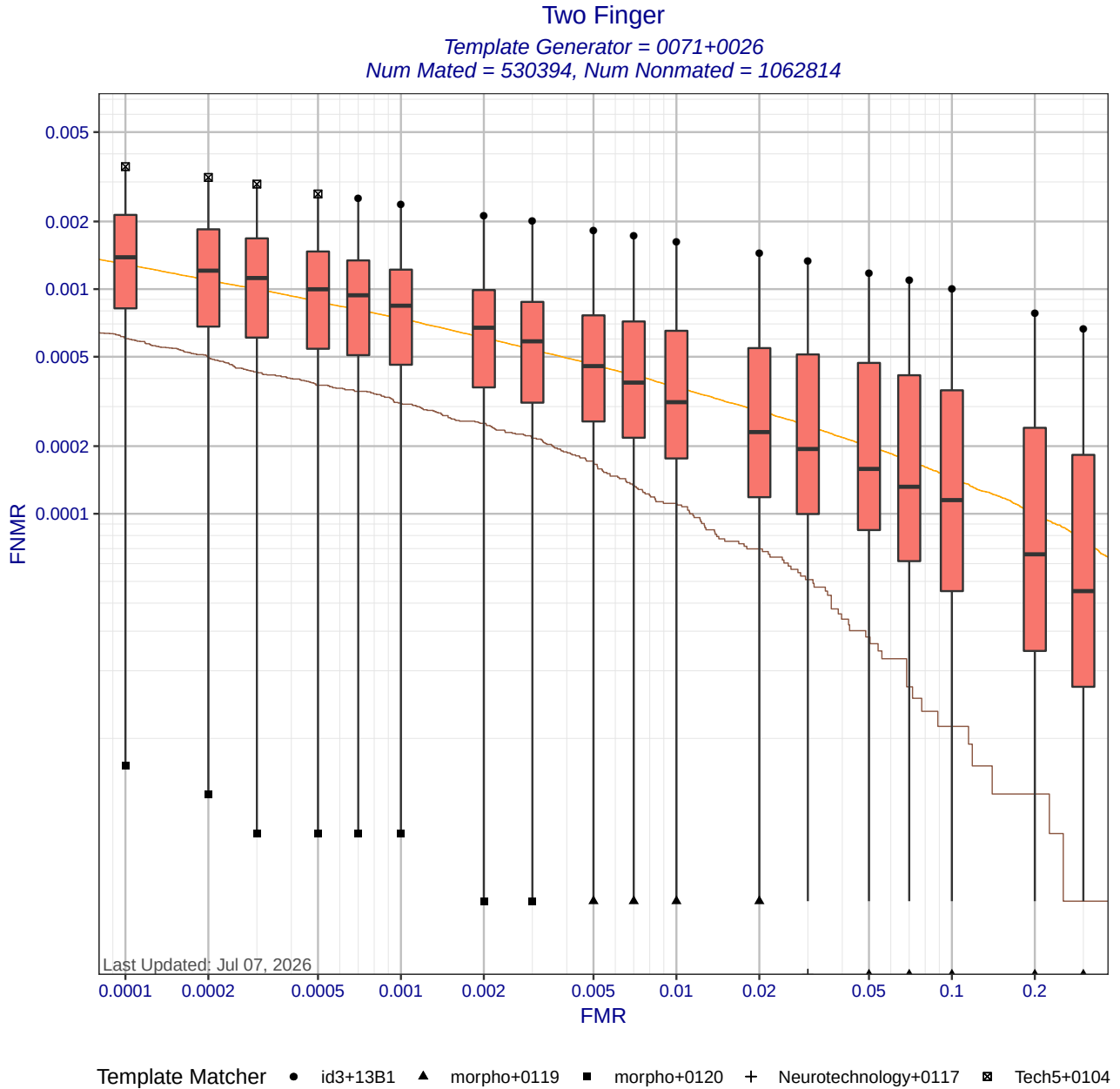
Figure 6: Two Finger DET statistics for template generator 0071+0026. Each box shows the distribution of FNMRs at a fixed FMR across different matchers. The whisker ends show the minimum and maximum FNMRs. The brown curve shows the DET curve when the matcher and template generators were submitted by the same participant. The orange DET curve shows pooled performance when all matchers use templates created by 0071+0026. Score-level fusion is achieved by averaging the scores for left and right index fingers.
