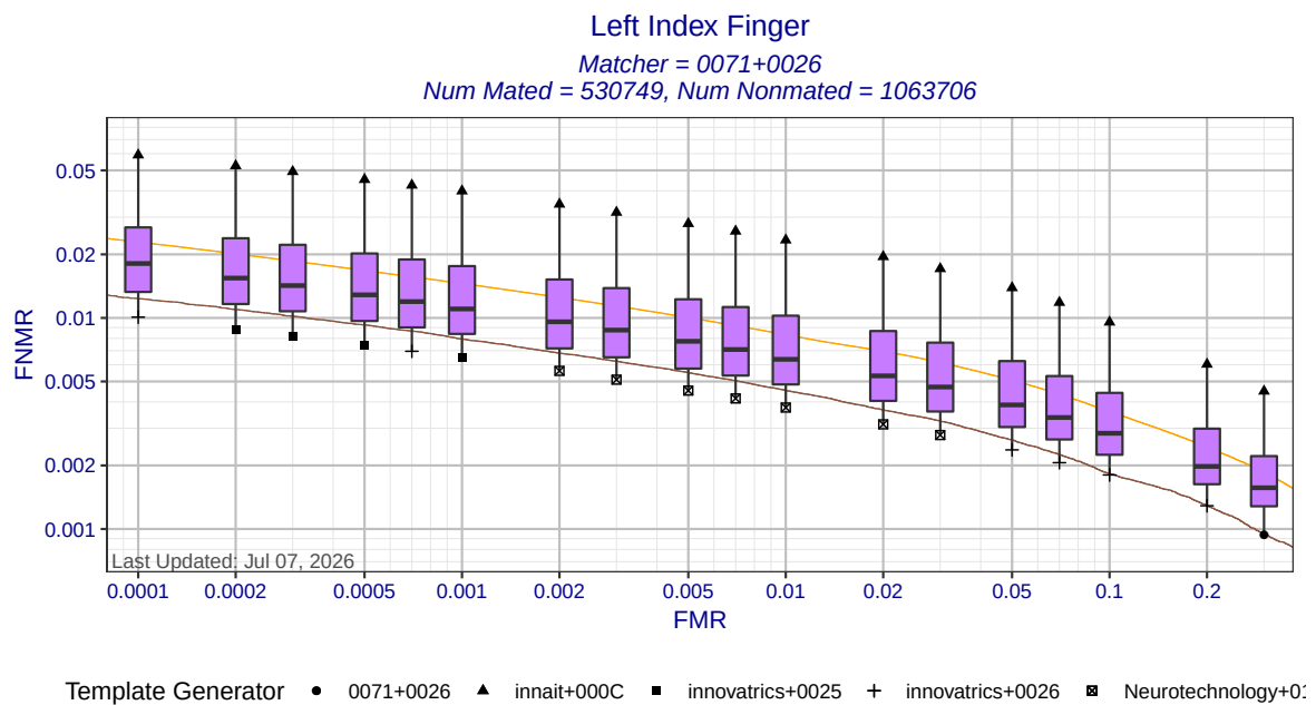
Figure 4: Left index finger DET statistics for matcher 0071+0026. Each box shows the distribution of FNMRs at a fixed FMR across all MINEX III compliant template generators. The ends of whiskers show the minimum and maximum FNMRs. The orange DET curve shows pooled performance against all template generators.
