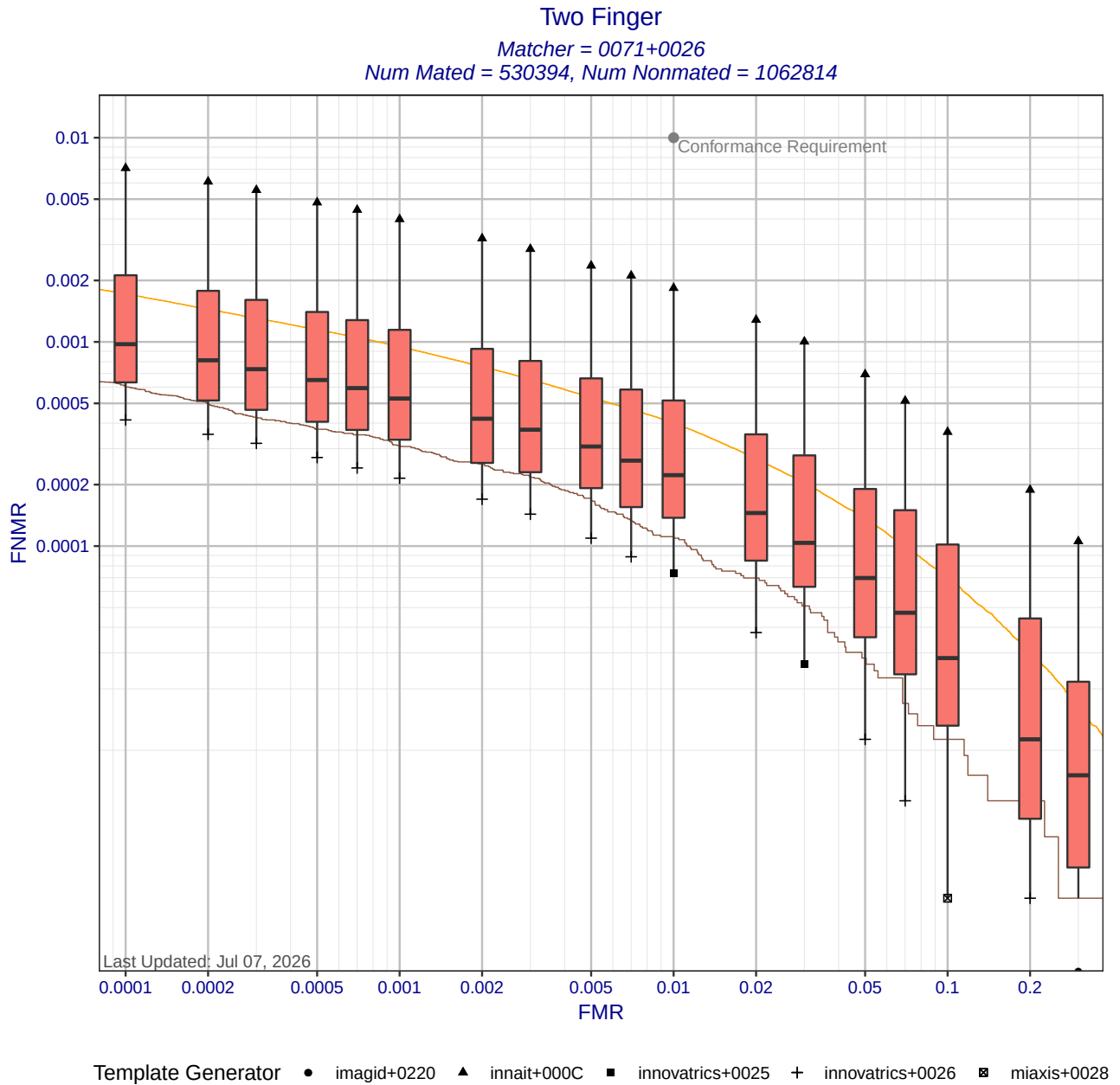
Figure 7: Two finger DET statistics for matcher 0071+0026. Each box shows the distribution of FNMRs at a fixed FMR across all MINEX III compliant template generators. The whisker ends show the minimum and maximum FNMRs. The orange DET curve shows pooled performance against all template generators. Score-level fusion is achieved by averaging the scores for left and right index fingers.
