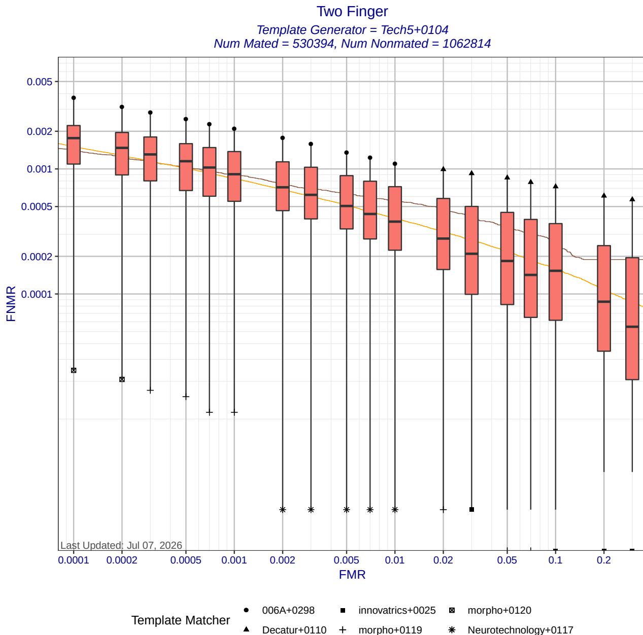
Figure 6: Two Finger DET statistics for template generator Tech5+0104. Each box shows the distribution of FNMNRs at a fixed FMR across different matchers. The whisker ends show the minimum and maximum FNMNRs. The brown curve shows the DET curve when the matcher and template generators were submitted by the same participant. The orange DET curve shows pooled performance when all matchers use templates created by Tech5+0104. Score-level fusion is achieved by averaging the scores for left and right index fingers.
