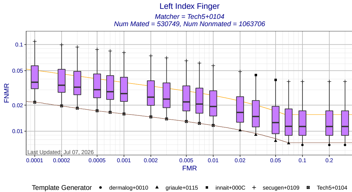
Figure 4: Left index finger DET statistics for matcher Tech5+0104. Each box shows the distribution of FNMRs at a fixed FMR across all MINEX III compliant template generators. The ends of the whiskers show the minimum and maximum FNMRs. The orange DET curve shows pooled performance against all template generators.
