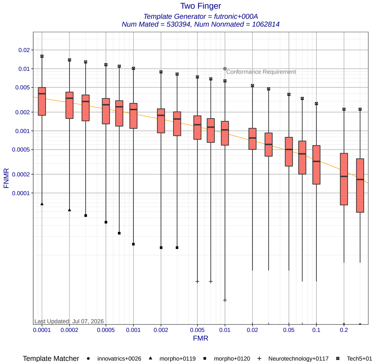
Figure 6: Two Finger DET statistics for template generator futronic+000A. Each box shows the distribution of FNMRs at a fixed FMR across different matchers. The whisker ends show the minimum and maximum FNMRs. The orange DET curve shows pooled performance when all matchers use templates created by futronic+000A. Score-level fusion is achieved by averaging the scores for left and right index fingers.
