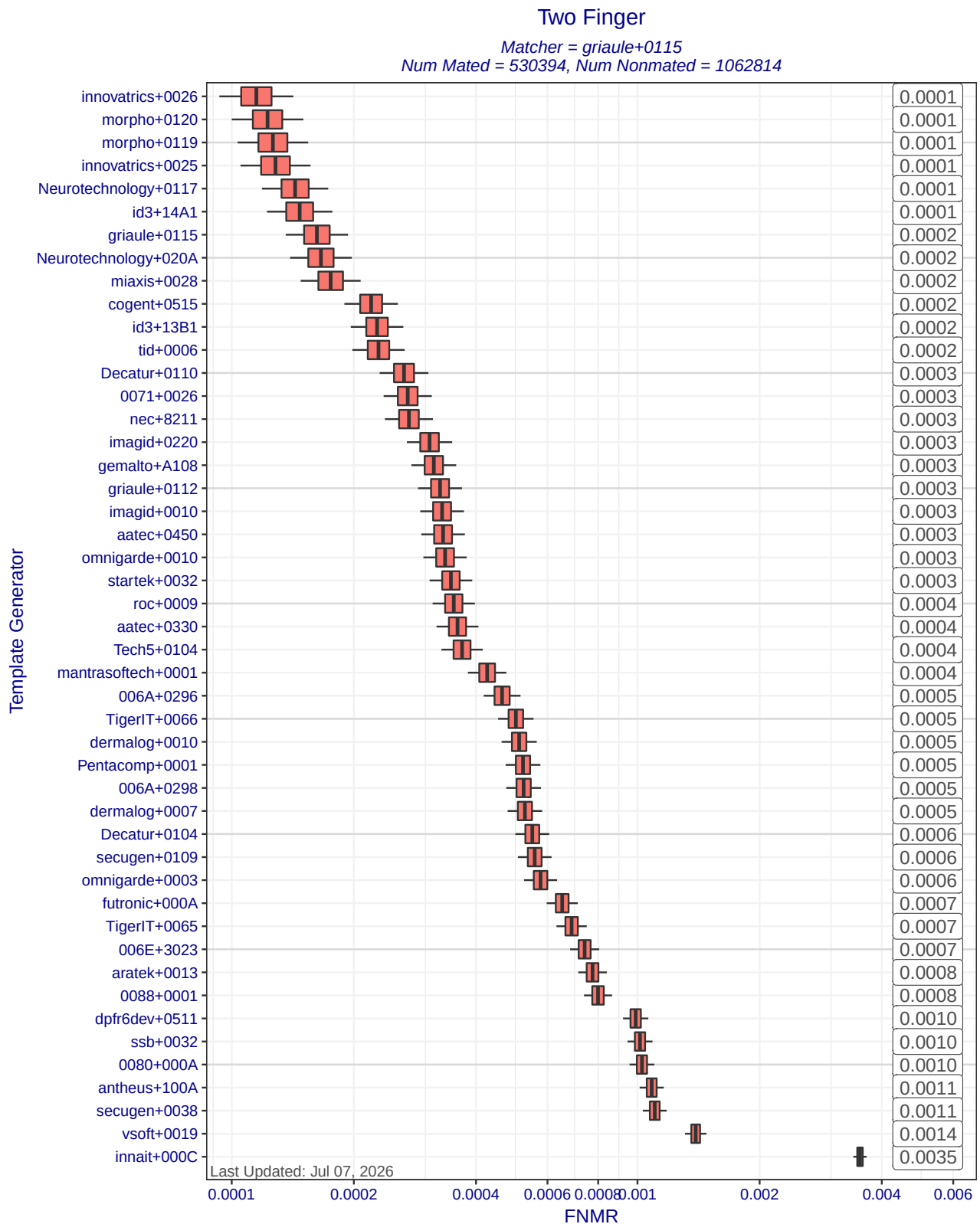
Figure 8: Two finger FNMR at FMR=0.01 when matcher griaule+0115 compares templates created by different template generators. Each box represents uncertainty about the true FNMR. The box edges mark the 50% confidence intervals while the whiskers mark the 90% confidence intervals. The numbers on the right show the actual computed FNMRs. Score-level fusion is achieved by averaging the scores for left and right index fingers.
