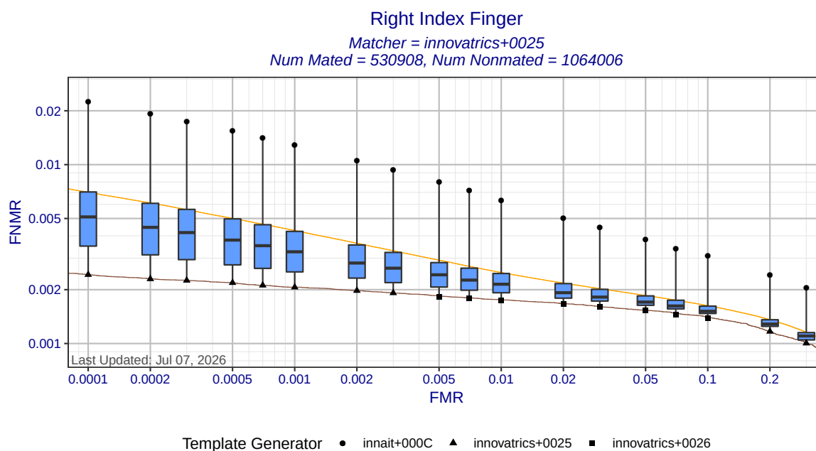
Figure 3: Right index finger DET statistics for matcher innovatrics+0025. Each box shows the distribution of FNR at a fixed FMR across all MINEX III compliant template generators. The ends of the whiskers show the minimum and maximum FNRs. The orange DET curve shows pooled performance against all template generators.
