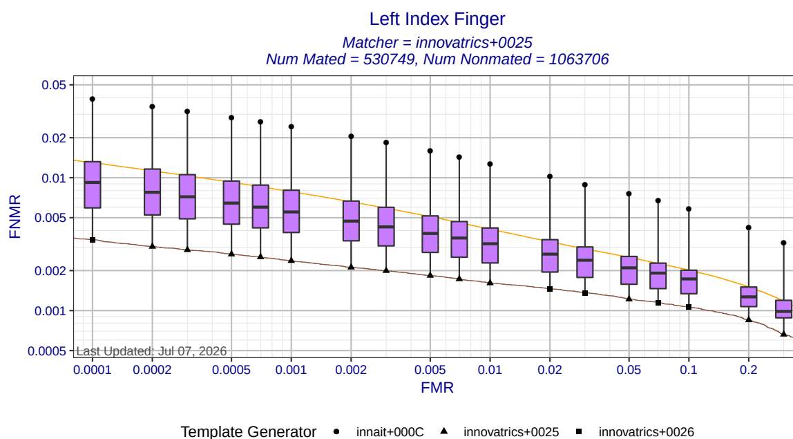
Figure 4: Left index finger DET statistics for matcher innovatrics+0025. Each box shows the distribution of FNRs at a fixed FMR across all MINEX III compliant template generators. The ends of the whiskers show the minimum and maximum FNRs. The orange DET curve shows pooled performance against all template generators.
