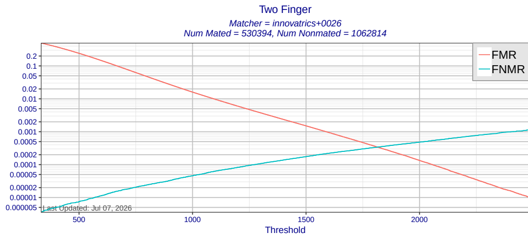
Figure 12: Two finger FMR and FNMR as a function of score threshold for matcher innovatrics+0026 using templates created by all MINEX III compliant template generators. Score-level fusion is achieved by averaging scores for the left and right index fingers.
