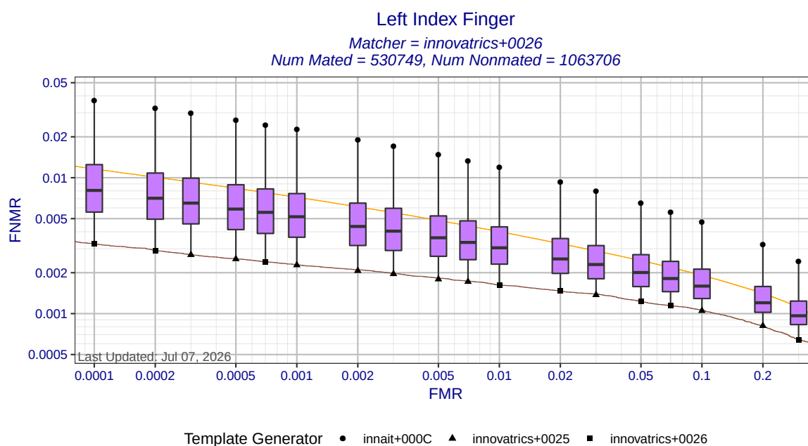
Figure 4: Left index finger DET statistics for matcher innovatrics+0026. Each box shows the distribution of FNMRs at a fixed FMR across all MINEX III compliant template generators. The ends of the whiskers show the minimum and maximum FNMRs. The orange DET curve shows pooled performance against all template generators.
