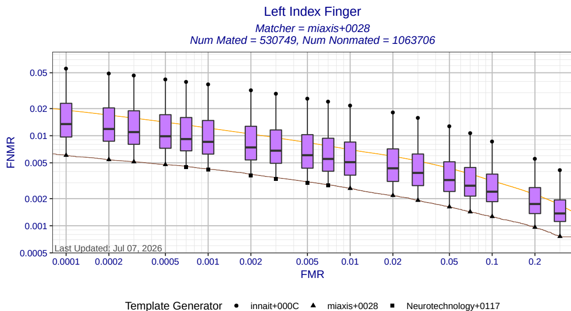
Figure 4: Left index finger DET statistics for matcher miaxis+0028. Each box shows the distribution of FNMRs at a fixed FMR across all MINEX III compliant template generators. The ends of whiskers show the minimum and maximum FNMRs. The orange DET curve shows pooled performance against all template generators.
