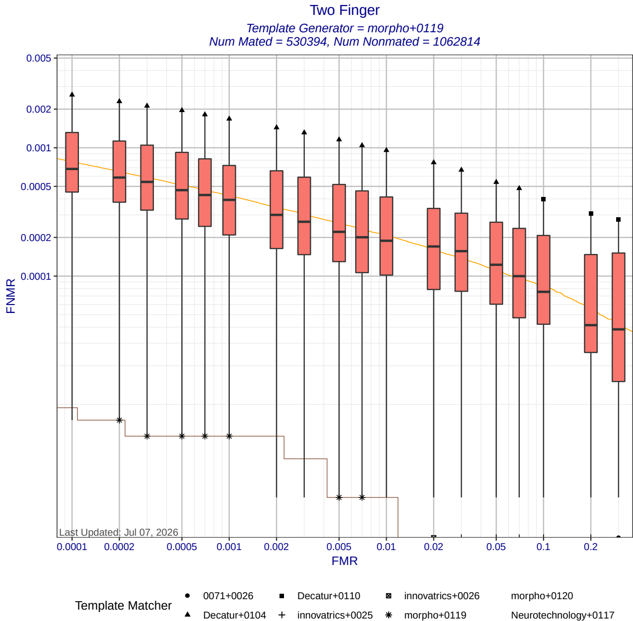
Figure 6: Two Finger DET statistics for template generator morpho+0119. Each box shows the distribution of FNMIRs at a fixed FMR across different matchers. The whisker ends show the minimum and maximum FNMIRs. The brown curve shows the DET curve when the matcher and template generators were submitted by the same participant. The orange DET curve shows pooled performance when all matchers use templates created by morpho+0119. Score-level fusion is achieved by averaging the scores for left and right index fingers.
