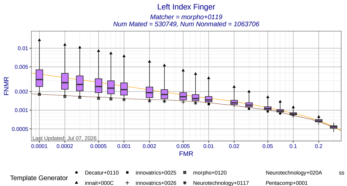
Figure 4: Left index finger DET statistics for matcher morpho+0119. Each box shows the distribution of FNMRs at a fixed FMR across all MINEX III compliant template generators. The ends of the whiskers show the minimum and maximum FNMRs. The orange DET curve shows pooled performance against all template generators.
