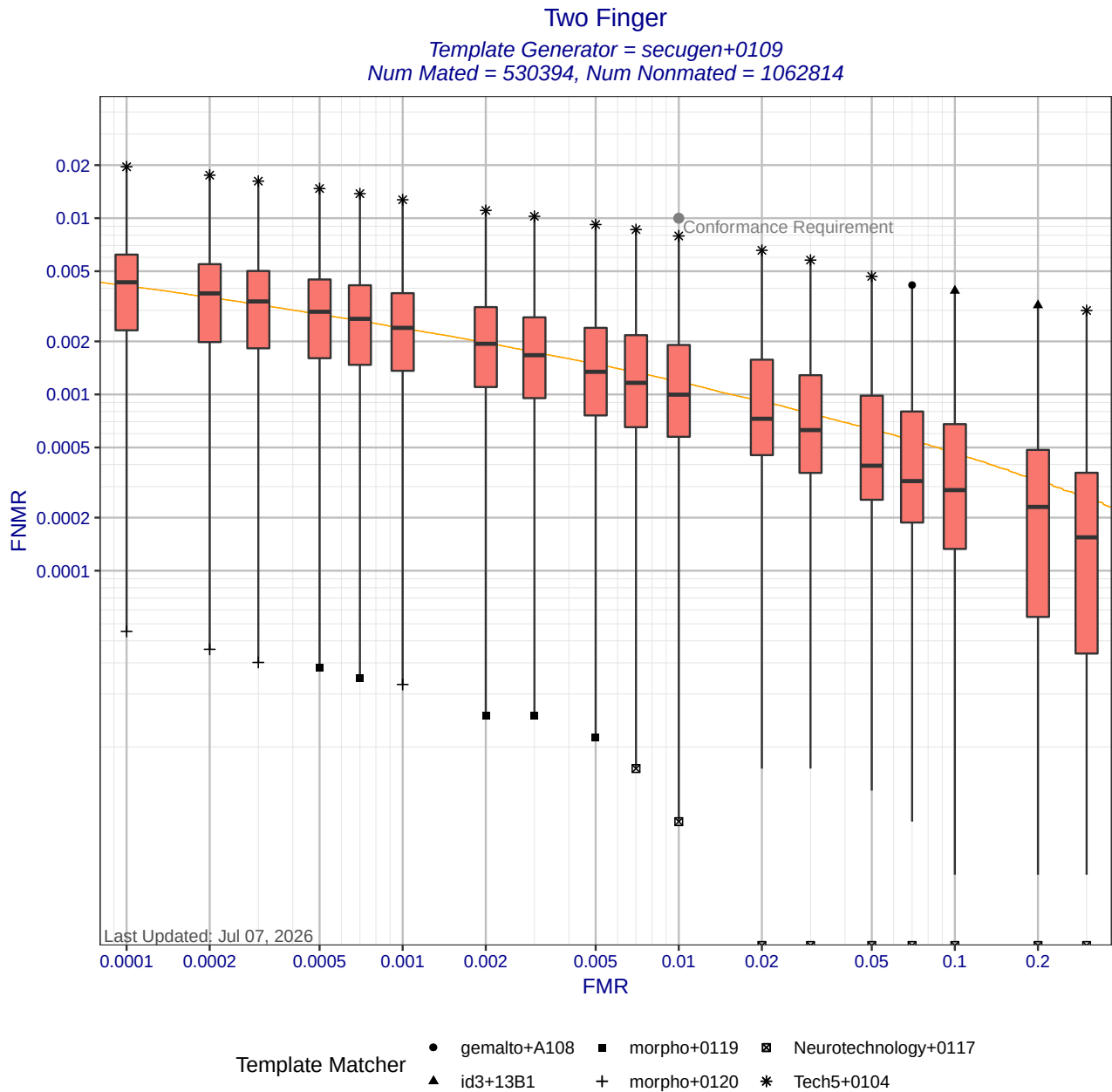
Figure 6: Two Finger DET statistics for template generator secugen+0109. Each box shows the distribution of FNMNRs at a fixed FMR across different matchers. The whisker ends show the minimum and maximum FNMNRs. The orange DET curve shows pooled performance when all matchers use templates created by secugen+0109. Score-level fusion is achieved by averaging the scores for left and right index fingers.
