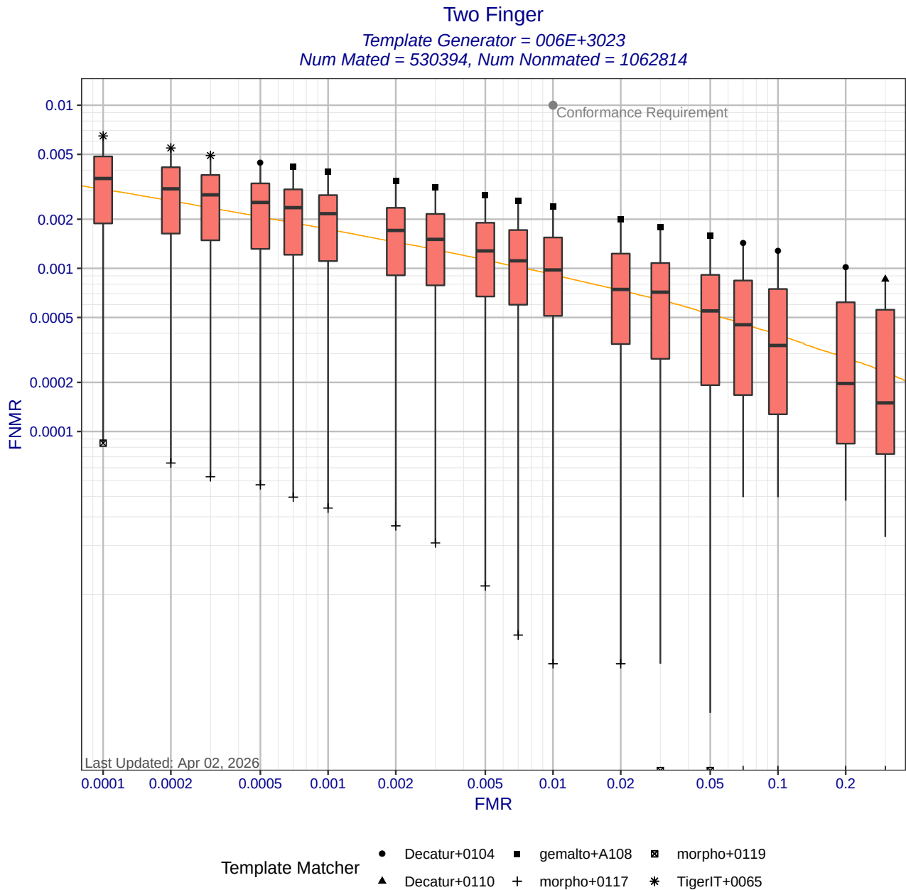
Figure 6: Two Finger DET statistics for template generator 006E+3023. Each box shows the distribution of FNMRs at a fixed FMR across different matchers. The whisker ends show the minimum and maximum FNMRs. The orange DET curve shows pooled performance when all matchers use templates created by 006E+3023. Score-level fusion is achieved by averaging the scores for left and right index fingers.
