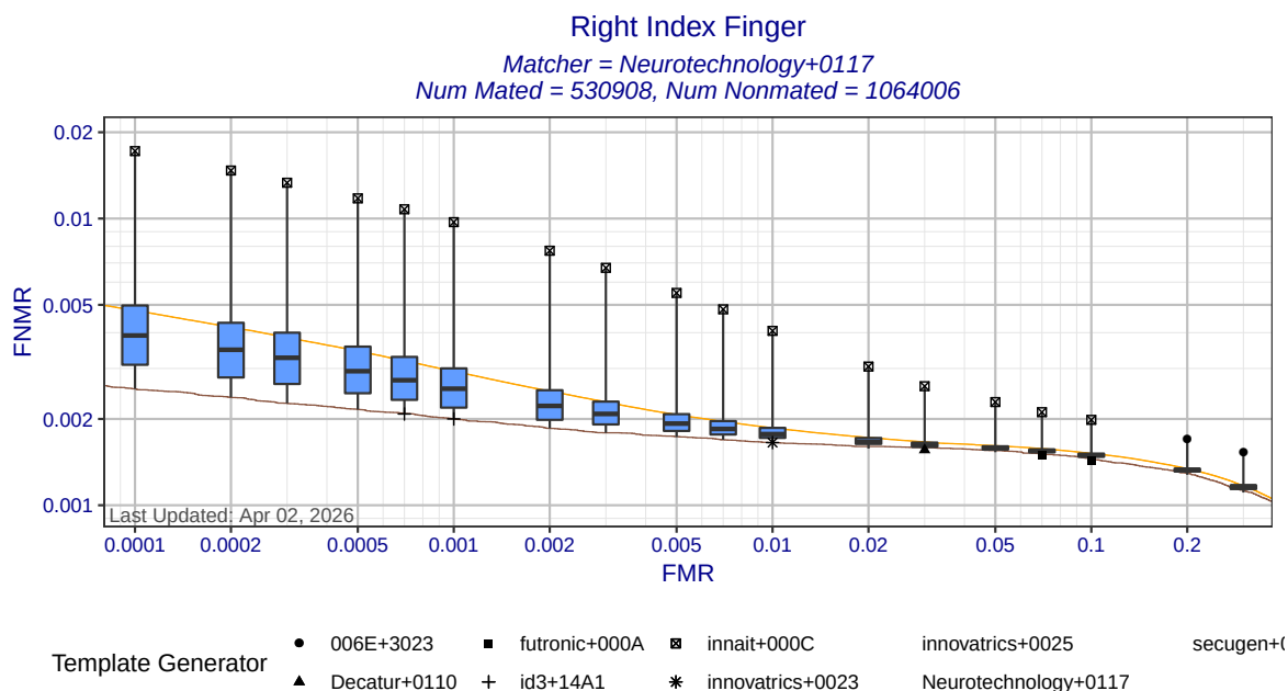
Figure 3: Right index finger DET statistics for matcher Neurotechnology+0117. Each box shows the distribution of FNMR at a fixed FMR across all MINEX III compliant template generators. The ends of the whiskers show the minimum and maximum FNMRs. The orange DET curve shows pooled performance against all template generators.
