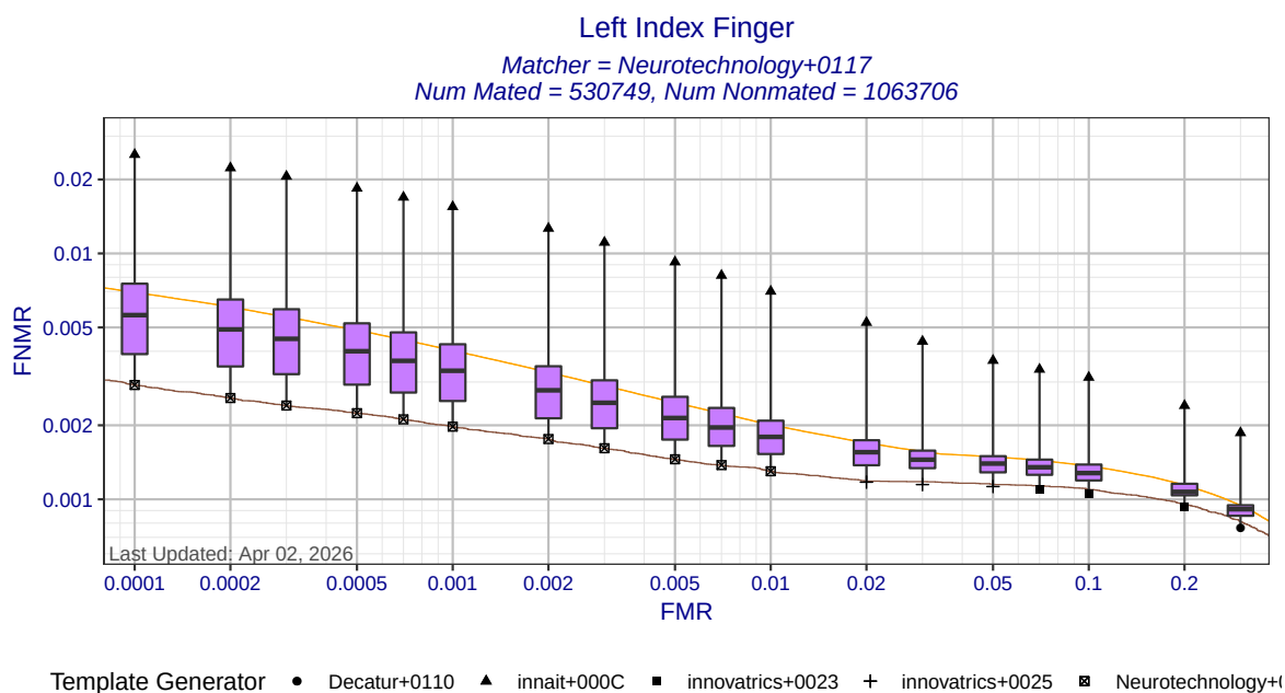
Figure 4: Left index finger DET statistics for matcher Neurotechnology+0117. Each box shows the distribution of FNMRs at a fixed FMR across all MINEX III compliant template generators. The ends of the whiskers show the minimum and maximum FNMRs. The orange DET curve shows pooled performance against all template generators.
