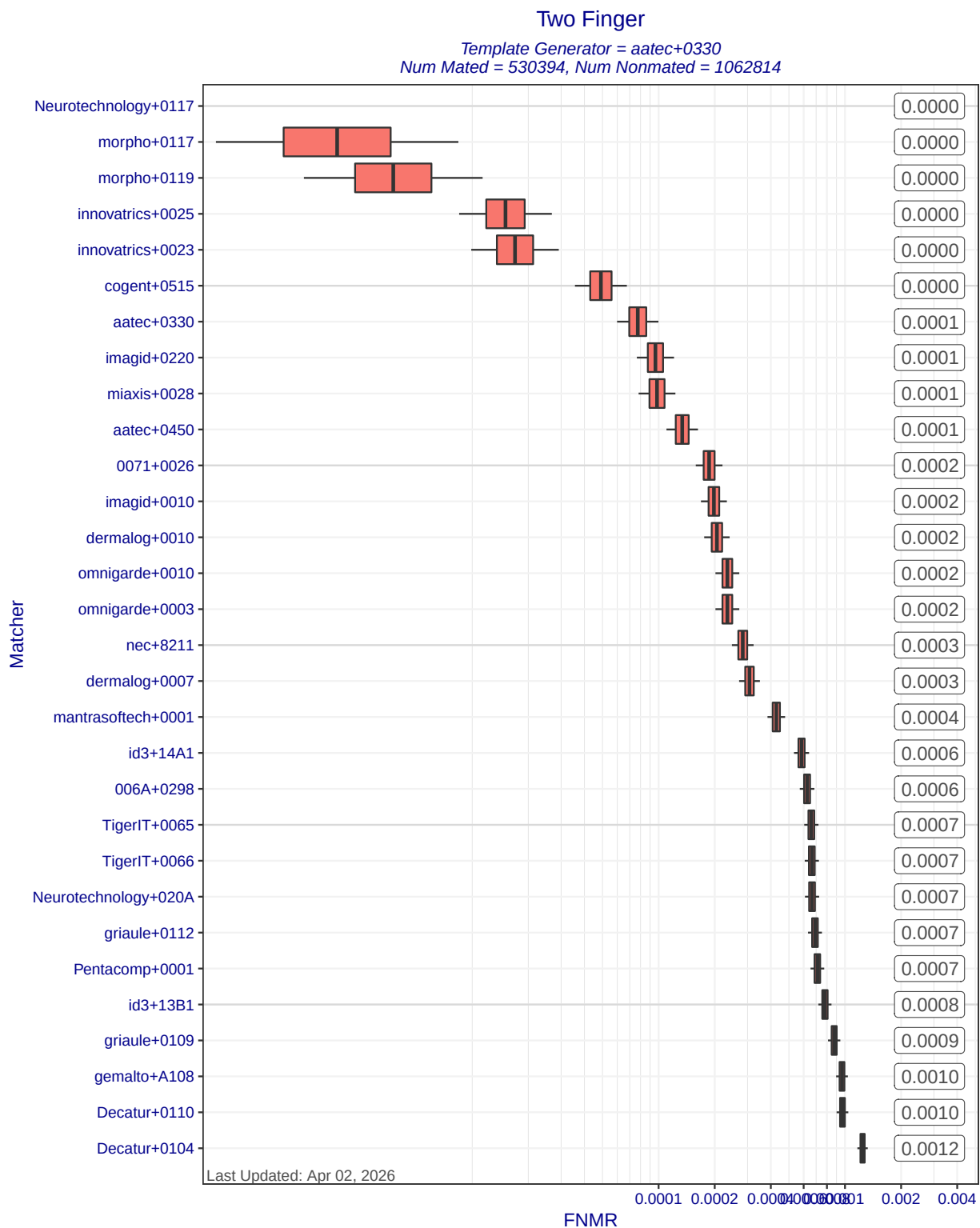
Figure 7: Two Finger FNMR at FMR=0.01 when different matchers compare templates created by template generator aatec+0330. Each box represents uncertainty about the true FNMR. The box edges mark the 50% confidence intervals while the whiskers mark the 90% confidence intervals. The numbers on the right show the actual computed FNMRs. Score-level fusion is achieved by averaging the scores for left and right index fingers.
