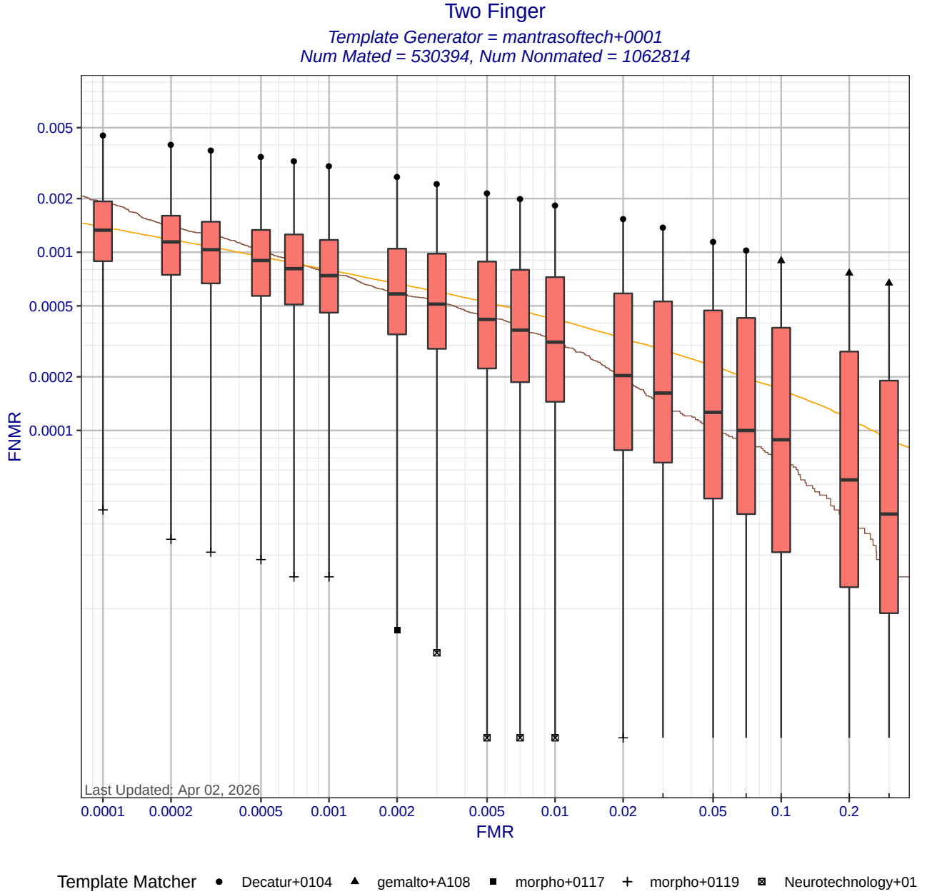
Figure 6: Two Finger DET statistics for template generator mantrasoftech+0001. Each box shows the distribution of FNMNRs at a fixed FMR across different matchers. The whisker ends show the minimum and maximum FNMNRs. The brown curve shows the DET curve when the matcher and template generators were submitted by the same participant. The orange DET curve shows pooled performance when all matchers use templates created by mantrasoftech+0001. Score-level fusion is achieved by averaging the scores for left and right index fingers.
