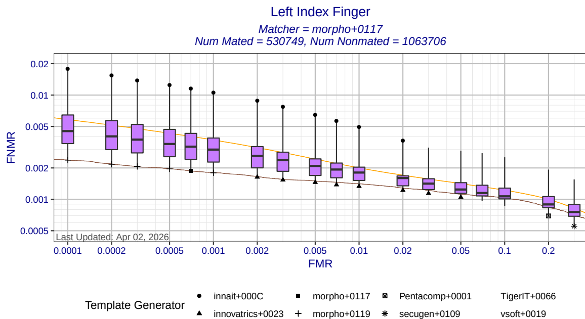
Figure 4: Left index finger DET statistics for matcher morpho+0117. Each box shows the distribution of FNMRs at a fixed FMR across all MINEX III compliant template generators. The ends of the whiskers show the minimum and maximum FNMRs. The orange DET curve shows pooled performance against all template generators.
