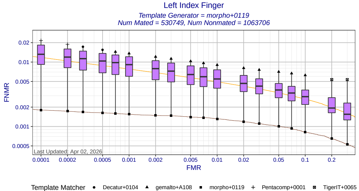
Figure 4: Left Index Finger DET statistics for template generator morpho+0119. Each box shows the distribution of FNMRs at a fixed FMR across different template generators. The brown curve shows the DET curve when the matcher and template generators were submitted by the same participant. The orange DET curve shows pooled performance when all matchers use templates created by morpho+0119.
