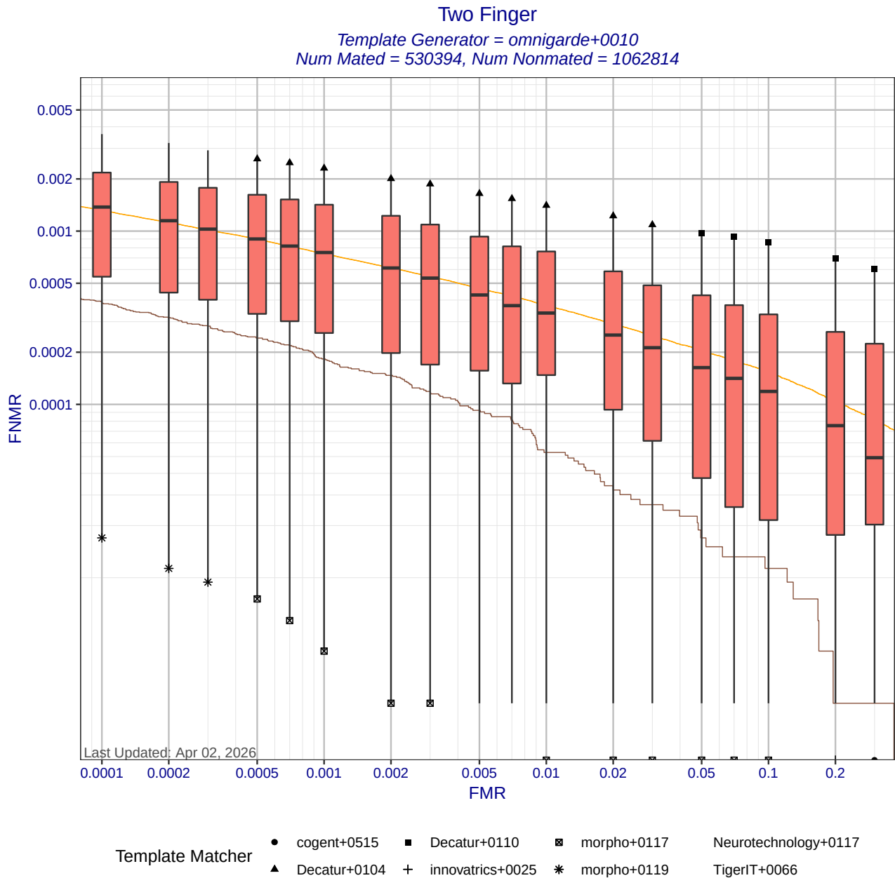
Figure 6: Two Finger DET statistics for template generator omnigarde+0010. Each box shows the distribution of FNMIRs at a fixed FMR across different matchers. The whisker ends show the minimum and maximum FNMIRs. The brown curve shows the DET curve when the matcher and template generators were submitted by the same participant. The orange DET curve shows pooled performance when all matchers use templates created by omnigarde+0010. Score-level fusion is achieved by averaging the scores for left and right index fingers.
