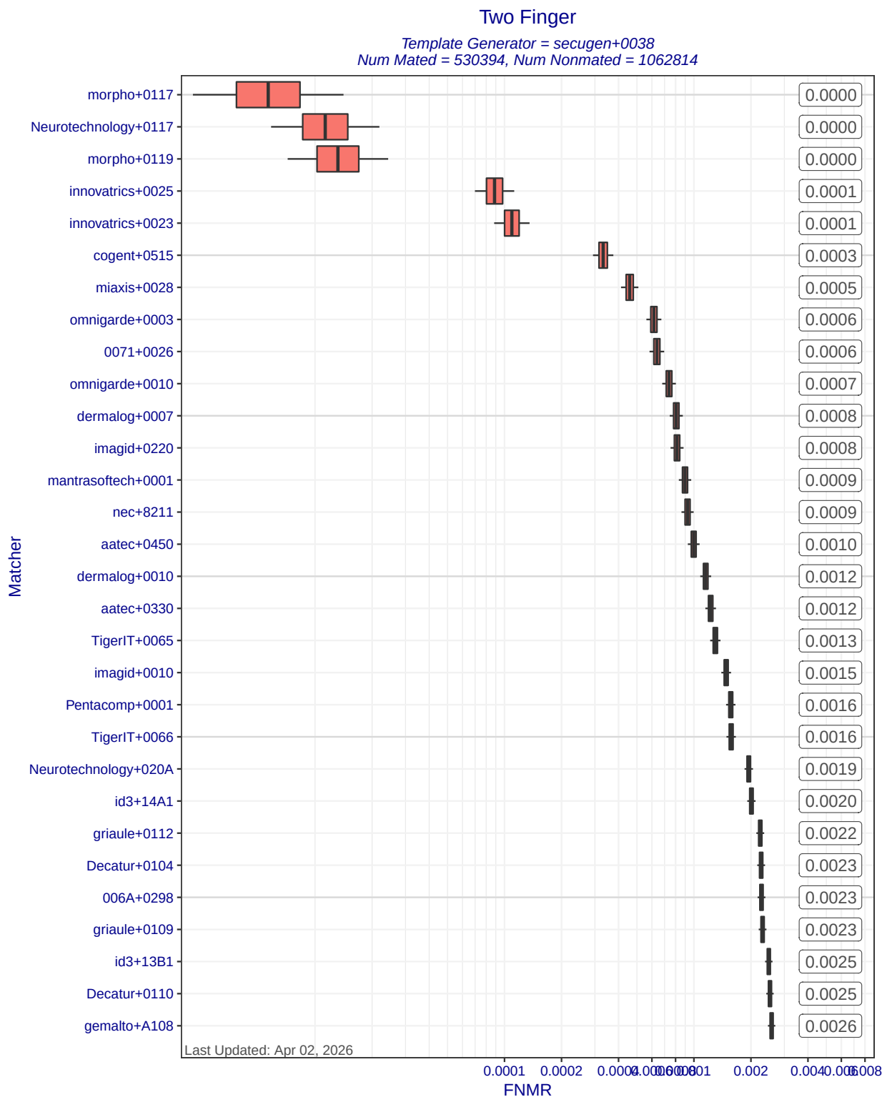
Figure 7: Two Finger FNMR at FMR=0.01 when different matchers compare templates created by template generator secugen+0038. Each box represents uncertainty about the true FNMR. The box edges mark the 50% confidence intervals while the whiskers mark the 90% confidence intervals. The numbers on the right show the actual computed FNMRs. Score-level fusion is achieved by averaging the scores for left and right index fingers.
