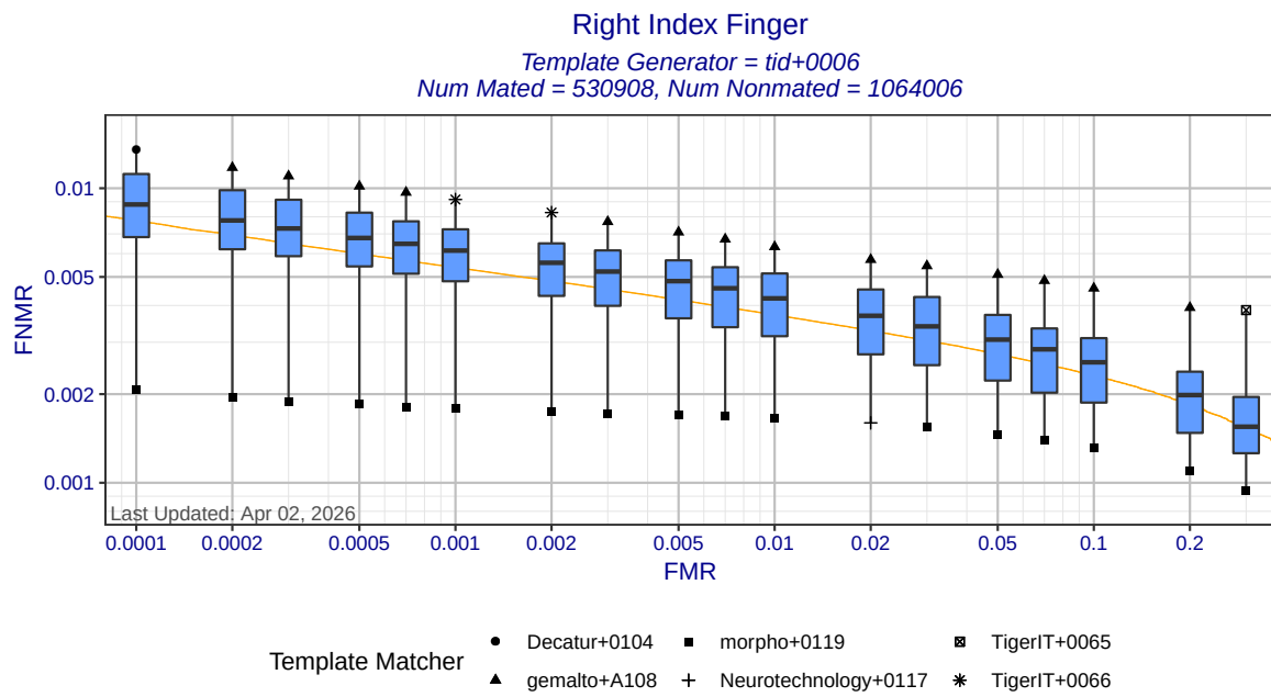
Figure 3: Right Index Finger DET statistics for template generator tid+0006. Each box shows the distribution of FNMRs at a fixed FMR across different matchers. The whisker ends show the minimum and maximum FNMRs. The orange DET curve shows pooled performance when all matchers use templates created by tid+0006.
