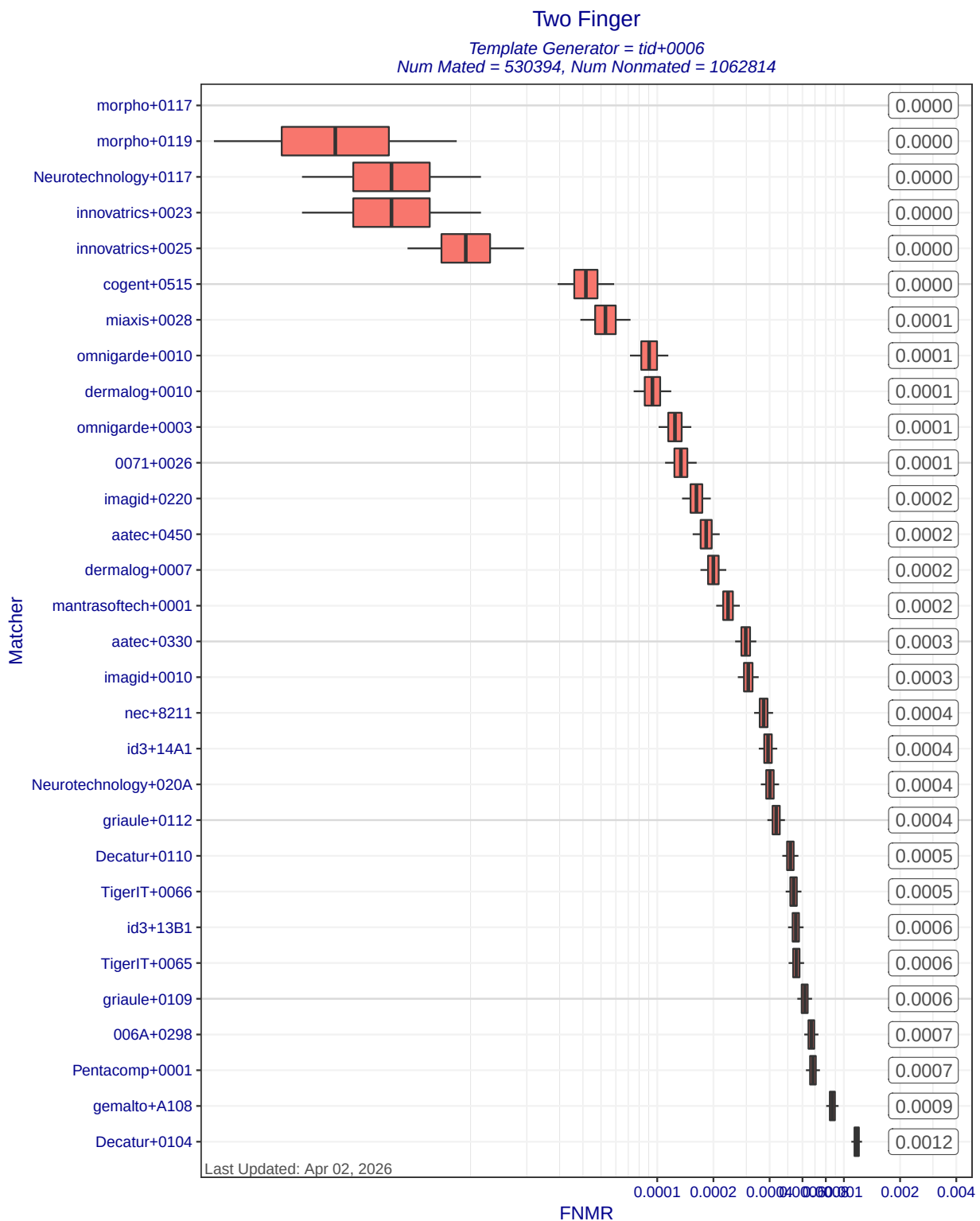
Figure 7: Two Finger FNMR at FMR=0.01 when different matchers compare templates created by template generator tid+0006. Each box represents uncertainty about the true FNMR. The box edges mark the 50% confidence intervals while the whiskers mark the 90% confidence intervals. The numbers on the right show the actual computed FNMRs. Score-level fusion is achieved by averaging the scores for left and right index fingers.
