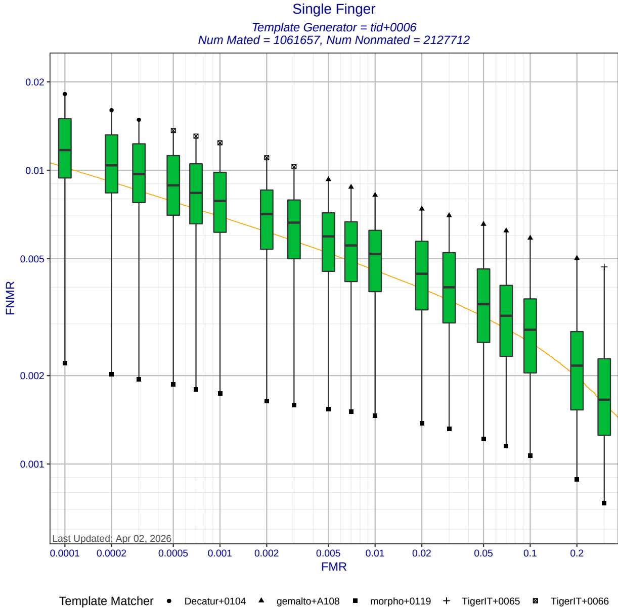
Figure 2: Single finger DET statistics for template generator tid+0006. Each box shows the distribution of FNMRs at a fixed FMR across different matchers. The whisker ends show the minimum and maximum FNMRs. The orange DET curve shows pooled performance when all matchers compare templates created by tid+0006.
