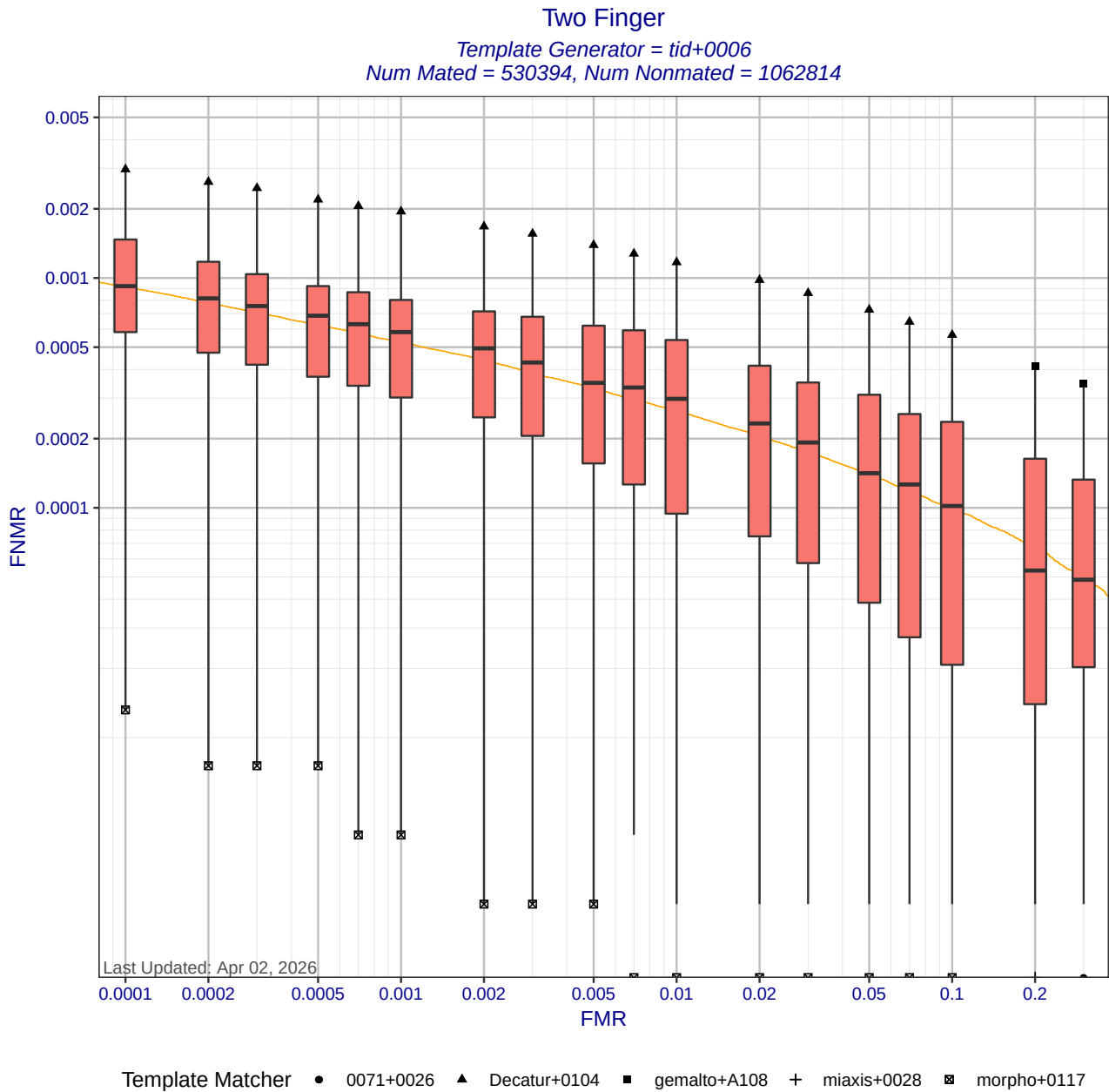
Figure 6: Two Finger DET statistics for template generator tid+0006. Each box shows the distribution of FNMNRs at a fixed FMR across different matchers. The whisker ends show the minimum and maximum FNMNRs. The orange DET curve shows pooled performance when all matchers use templates created by tid+0006. Score-level fusion is achieved by averaging the scores for left and right index fingers.
