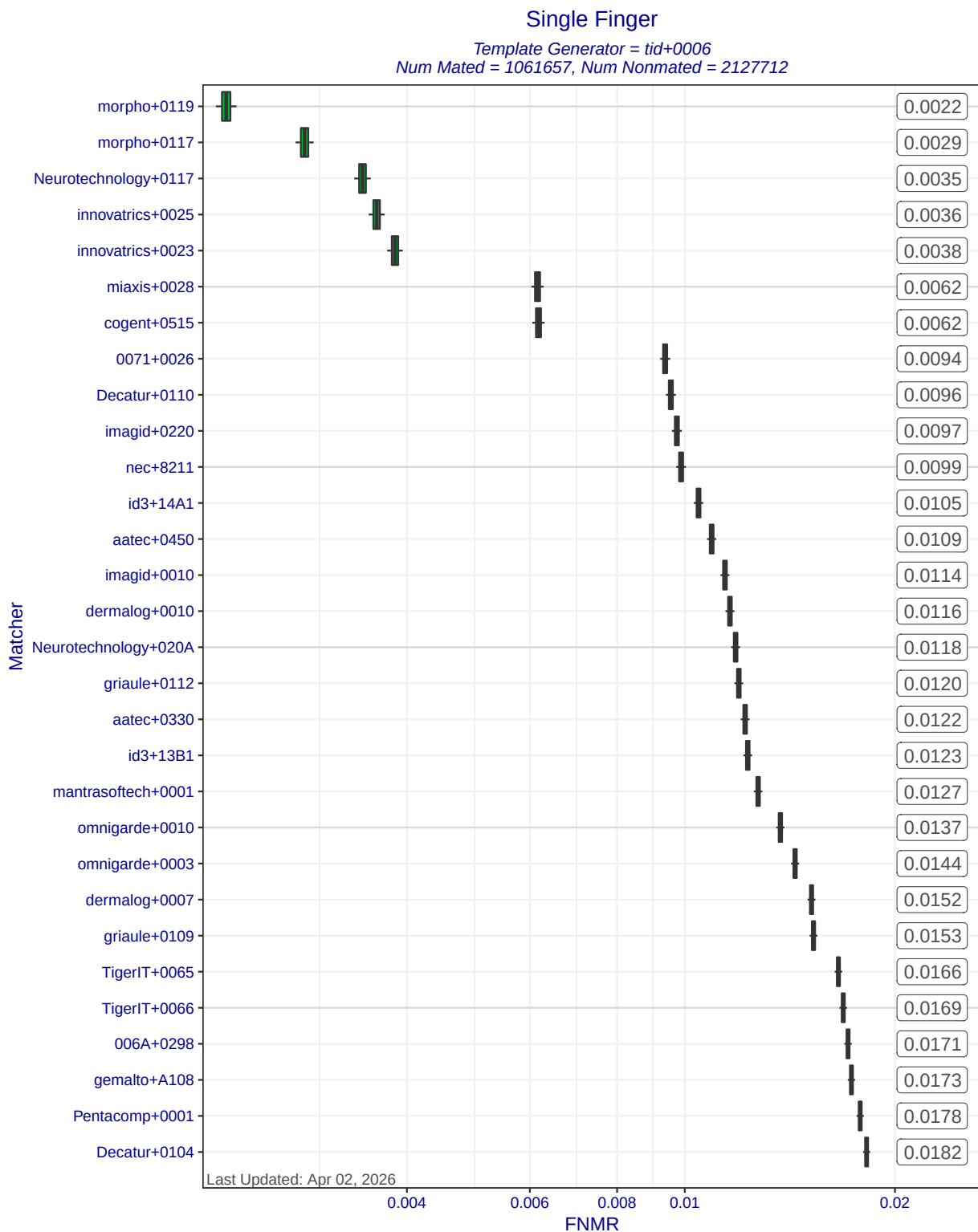
Figure 5: Single Finger FNMRs at FMR=0.0001 when MINEX III compliant matchers compare templates created by template generator tid+0006. Each box represents uncertainty about the true FNMR. The box edges mark the 50% confidence intervals while the whiskers mark the 90% confidence intervals. The numbers on the right show the actual computed FNMRs.
