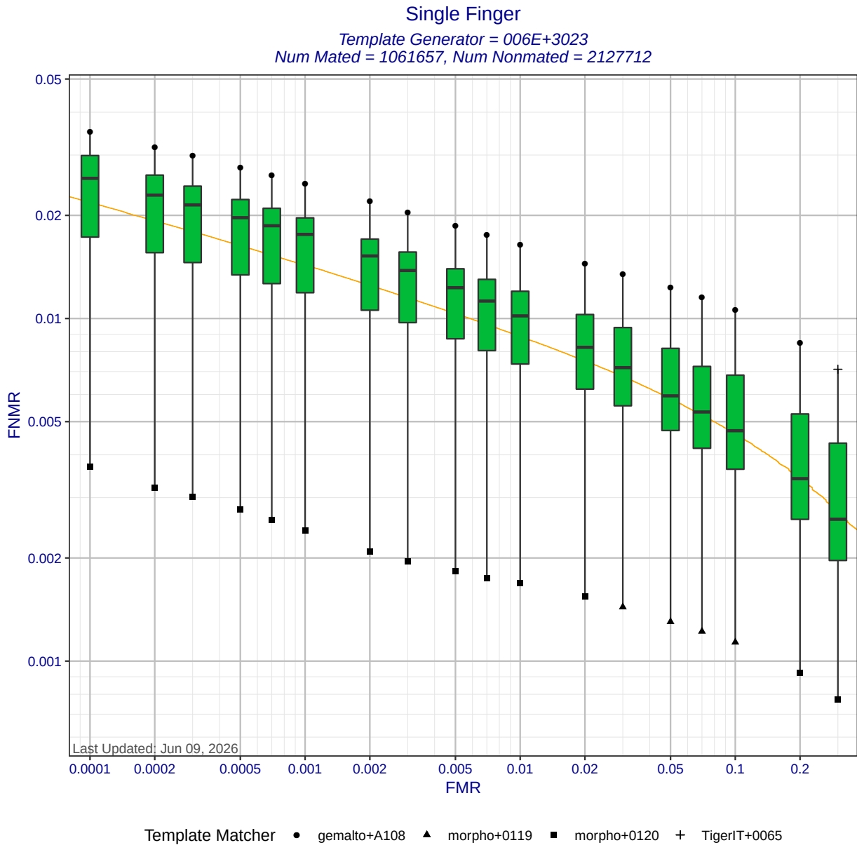
Figure 2: Single finger DET statistics for template generator 006E+3023. Each box shows the distribution of FNMRs at a fixed FMR across different matchers. The whisker ends show the minimum and maximum FNMRs. The orange DET curve shows pooled performance when all matchers compare templates created by 006E+3023.
