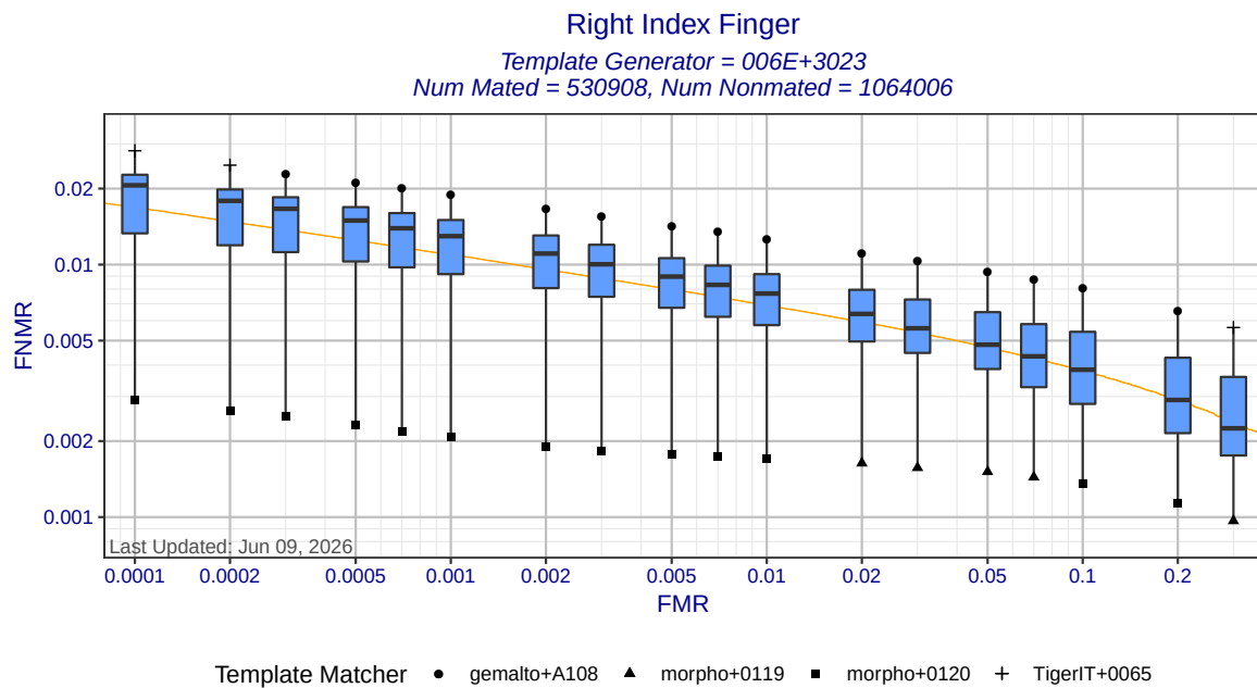
Figure 3: Right Index Finger DET statistics for template generator 006E+3023. Each box shows the distribution of FNMRs at a fixed FMR across different matchers. The whisker ends show the minimum and maximum FNMRs. The orange DET curve shows pooled performance when all matchers use templates created by 006E+3023.
