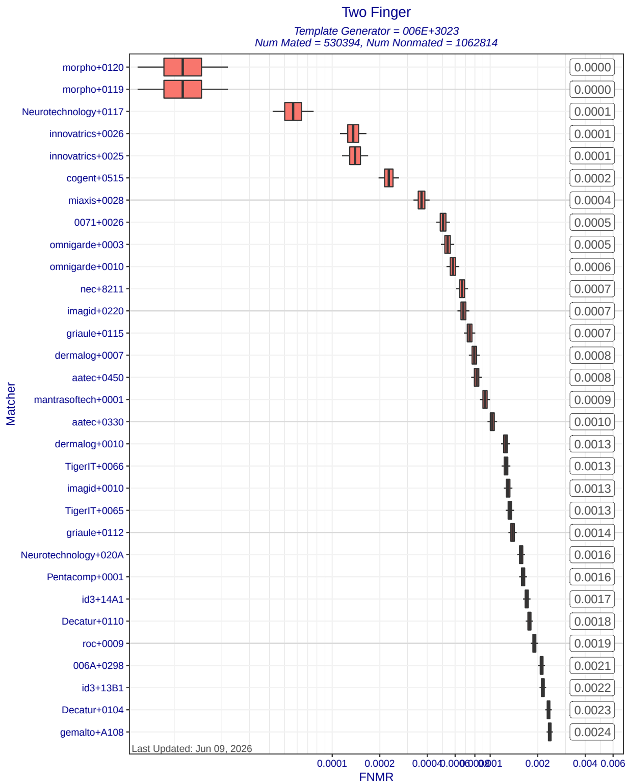
Figure 7: Two Finger FNMR at FMR=0.01 when different matchers compare templates created by template generator 006E+3023. Each box represents uncertainty about the true FNMR. The box edges mark the 50% confidence intervals while the whiskers mark the 90% confidence intervals. The numbers on the right show the actual computed FNMRs. Score-level fusion is achieved by averaging the scores for left and right index fingers.
