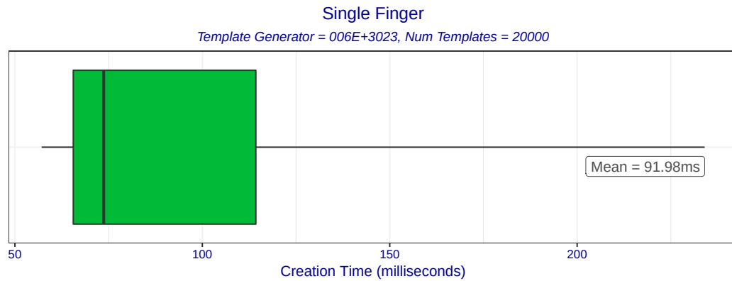
Figure 8: Boxplot of template creation times for template generator 006E+3023. The box edges mark the 10th and 90th percentiles while the whiskers mark the maximum and minimum creation times.
