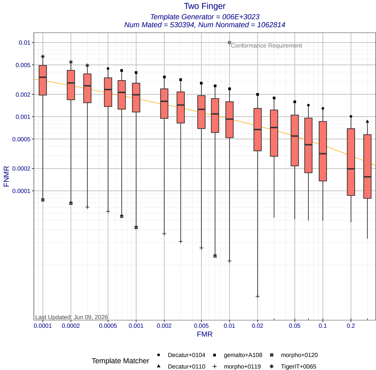
Figure 6: Two Finger DET statistics for template generator 006E+3023. Each box shows the distribution of FNRs at a fixed FMR across different matchers. The whisker ends show the minimum and maximum FNRs. The orange DET curve shows pooled performance when all matchers use templates created by 006E+3023. Score-level fusion is achieved by averaging the scores for left and right index fingers.
