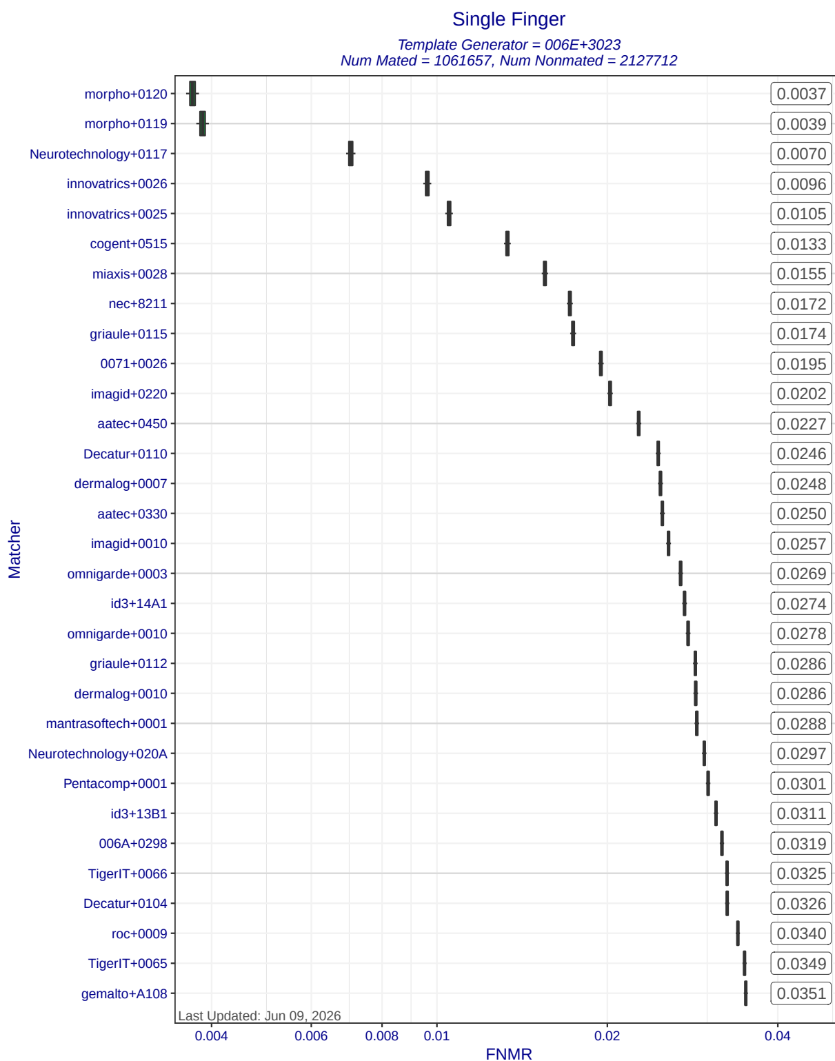
Figure 5: Single Finger FNMRs at FMR=0.0001 when MINEX III compliant matchers compare templates created by template generator 006E+3023. Each box represents uncertainty about the true FNMR. The box edges mark the 50% confidence intervals while the whiskers mark the 90% confidence intervals. The numbers on the right show the actual computed FNMRs.
