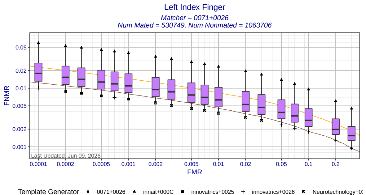
Figure 4: Left index finger DET statistics for matcher 0071+0026. Each box shows the distribution of FNMRs at a fixed FMR across all MINEX III compliant template generators. The ends of the whiskers show the minimum and maximum FNMRs. The orange DET curve shows pooled performance against all template generators.
