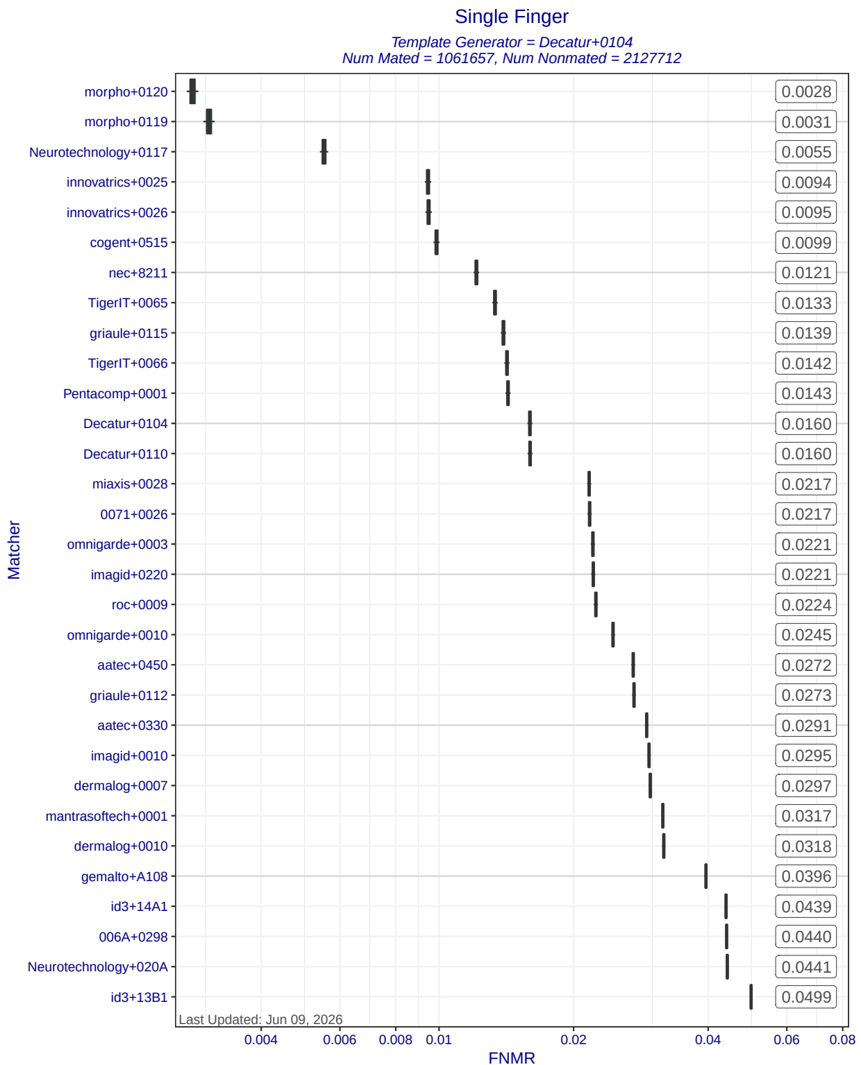
Figure 5: Single Finger FNMRS at FMR=0.0001 when MINEX III compliant matchers compare templates created by template generator Decatur+0104. Each box represents uncertainty about the true FNMRS. The box edges mark the 50% confidence intervals while the whiskers mark the 90% confidence intervals. The numbers on the right show the actual computed FNMRS.
