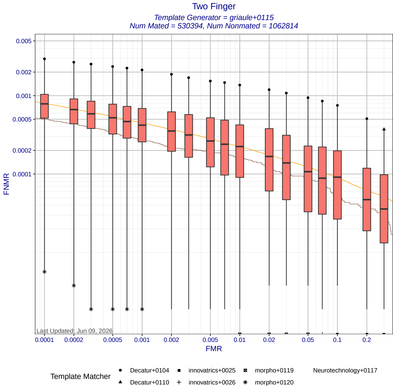
Figure 6: Two Finger DET statistics for template generator griaule+0115. Each box shows the distribution of FNMNRs at a fixed FMR across different matchers. The whisker ends show the minimum and maximum FNMNRs. The brown curve shows the DET curve when the matcher and template generators were submitted by the same participant. The orange DET curve shows pooled performance when all matchers use templates created by griaule+0115. Score-level fusion is achieved by averaging the scores for left and right index fingers.
