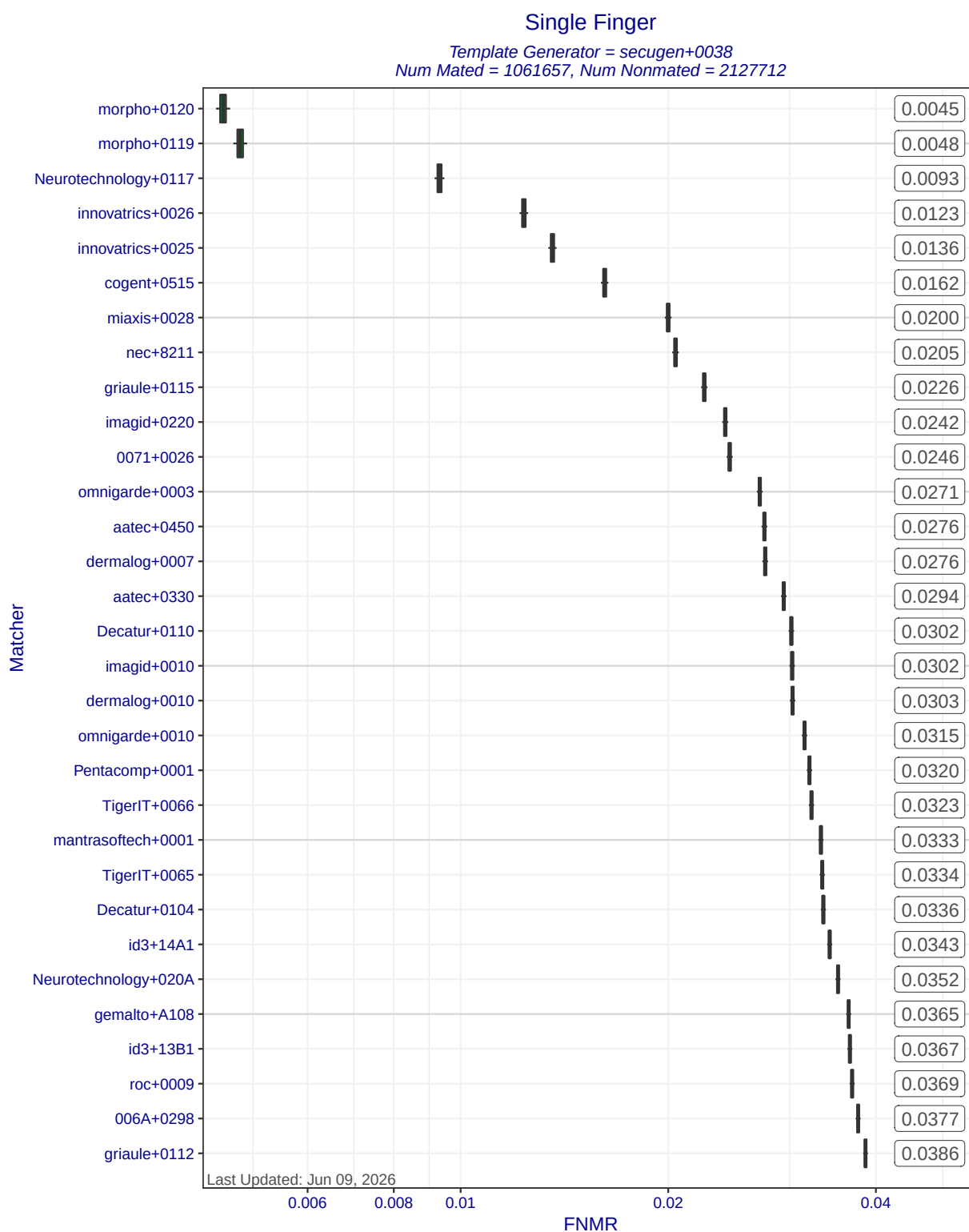
Figure 5: Single Finger FNMNRs at FMR=0.0001 when MINEX III compliant matchers compare templates created by template generator secugen+0038. Each box represents uncertainty about the true FNMNR. The box edges mark the 50% confidence intervals while the whiskers mark the 90% confidence intervals. The numbers on the right show the actual computed FNMNRs.
