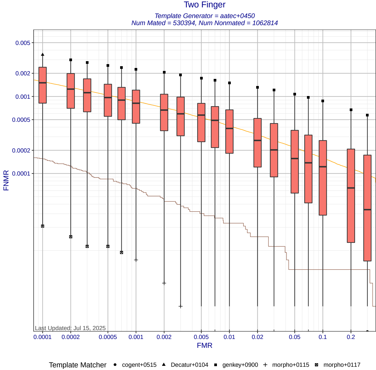
Figure 6: Two Finger DET statistics for template generator aatec+0450. Each box shows the distribution of FNMIRs at a fixed FMR across different matchers. The whisker ends show the minimum and maximum FNMIRs. The brown curve shows the DET curve when the matcher and template generators were submitted by the same participant. The orange DET curve shows pooled performance when all matchers use templates created by aatec+0450. Score-level fusion is achieved by averaging the scores for left and right index fingers.
