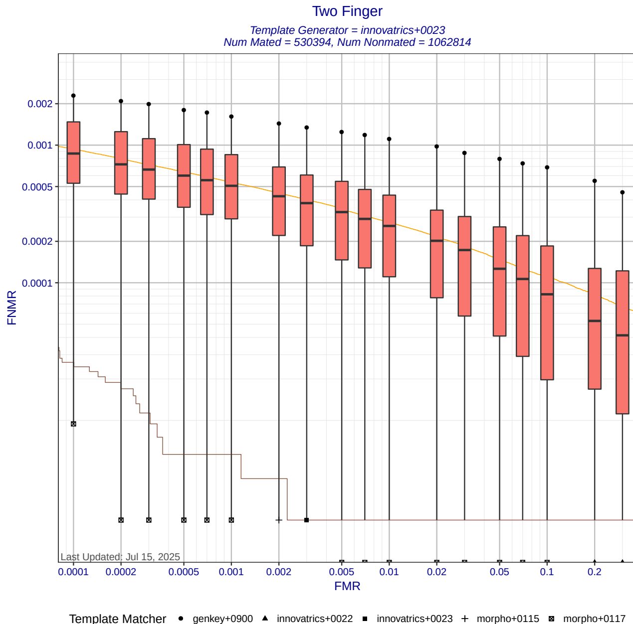
Figure 6: Two Finger DET statistics for template generator innovatrics+0023. Each box shows the distribution of FNMIRs at a fixed FMR across different matchers. The whisker ends show the minimum and maximum FNMIRs. The brown curve shows the DET curve when the matcher and template generators were submitted by the same participant. The orange DET curve shows pooled performance when all matchers use templates created by innovatrics+0023. Score-level fusion is achieved by averaging the scores for left and right index fingers.
