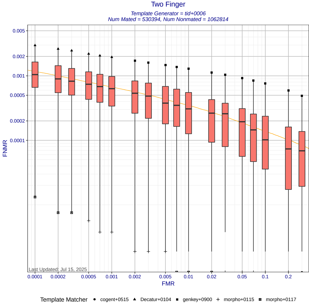
Figure 6: Two Finger DET statistics for template generator tid+0006. Each box shows the distribution of FNMRs at a fixed FMR across different matchers. The whisker ends show the minimum and maximum FNMRs. The orange DET curve shows pooled performance when all matchers use templates created by tid+0006. Score-level fusion is achieved by averaging the scores for left and right index fingers.
