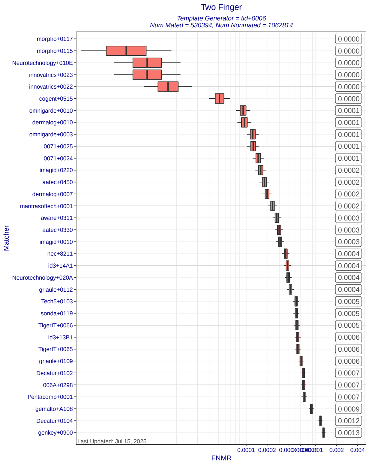
Figure 7: Two Finger FNMR at FMR=0.01 when different matchers compare templates created by template generator tid+0006. Each box represents uncertainty about the true FNMR. The box edges mark the 50% confidence intervals while the whiskers mark the 90% confidence intervals. The numbers on the right show the actual computed FNMRs. Score-level fusion is achieved by averaging the scores for left and right index fingers.
