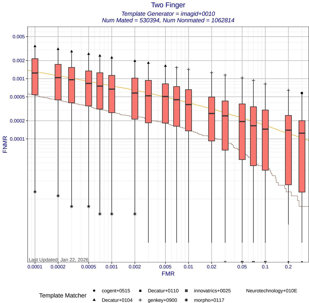
Figure 6: Two Finger DET statistics for template generator imagid+0010. Each box shows the distribution of FNMNRs at a fixed FMR across different matchers. The whisker ends show the minimum and maximum FNMNRs. The brown curve shows the DET curve when the matcher and template generators were submitted by the same participant. The orange DET curve shows pooled performance when all matchers use templates created by imagid+0010. Score-level fusion is achieved by averaging the scores for left and right index fingers.
