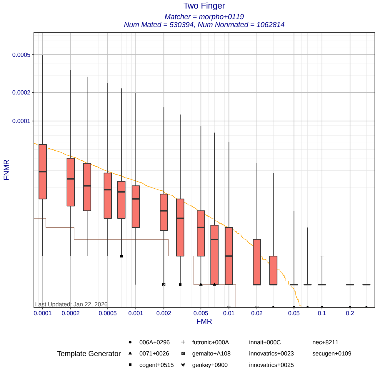
Figure 7: Two finger DET statistics for matcher morpho+0119. Each box shows the distribution of FNMRs at a fixed FMR across all MINEX III compliant template generators. The whisker ends show the minimum and maximum FNMRs. The orange DET curve shows pooled performance against all template generators. Score-level fusion is achieved by averaging the scores for left and right index fingers.
