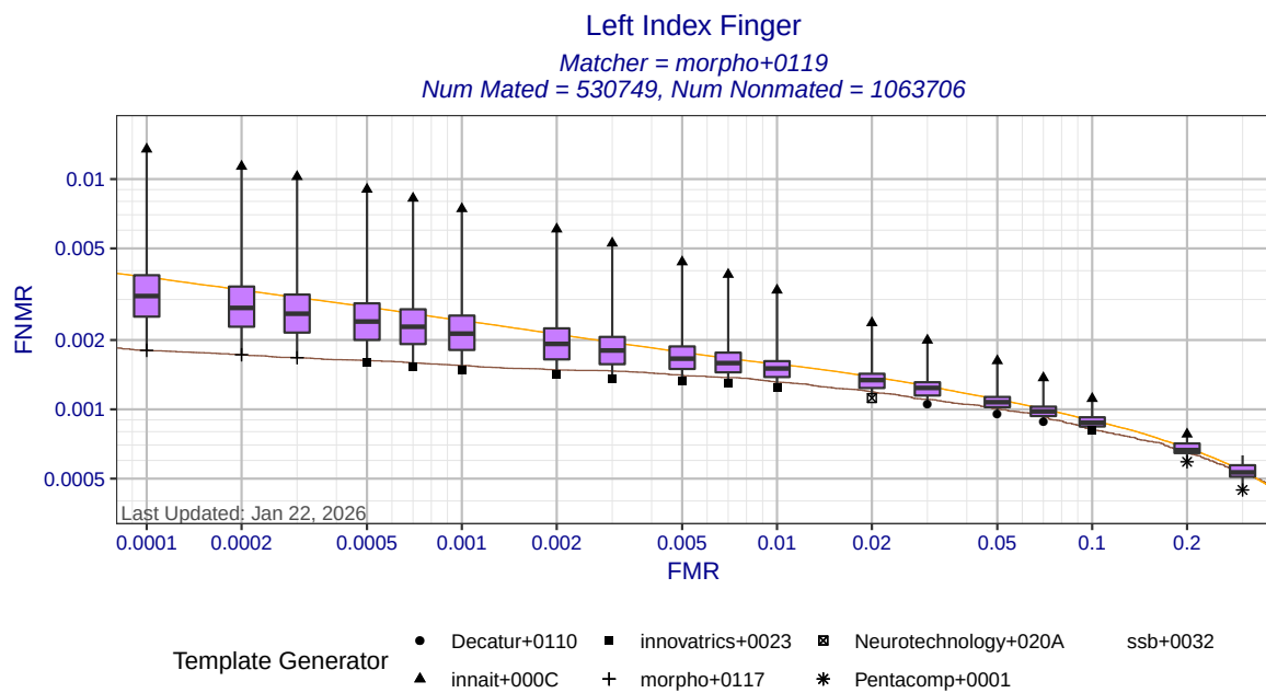
Figure 4: Left index finger DET statistics for matcher morpho+0119. Each box shows the distribution of FNMRs at a fixed FMR across all MINEX III compliant template generators. The ends of the whiskers show the minimum and maximum FNMRs. The orange DET curve shows pooled performance against all template generators.
