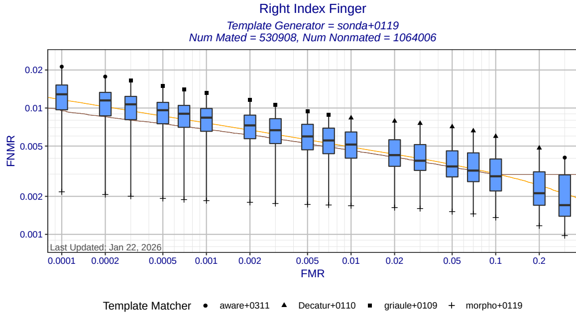
Figure 3: Right Index Finger DET statistics for template generator sonda+0119. Each box shows the distribution of FNMNRs at a fixed FMR across different matchers. The whisker ends show the minimum and maximum FNMNRs. The brown curve shows the DET curve when the matcher and template generators were submitted by the same participant. The orange DET curve shows pooled performance when all matchers use templates created by sonda+0119.
