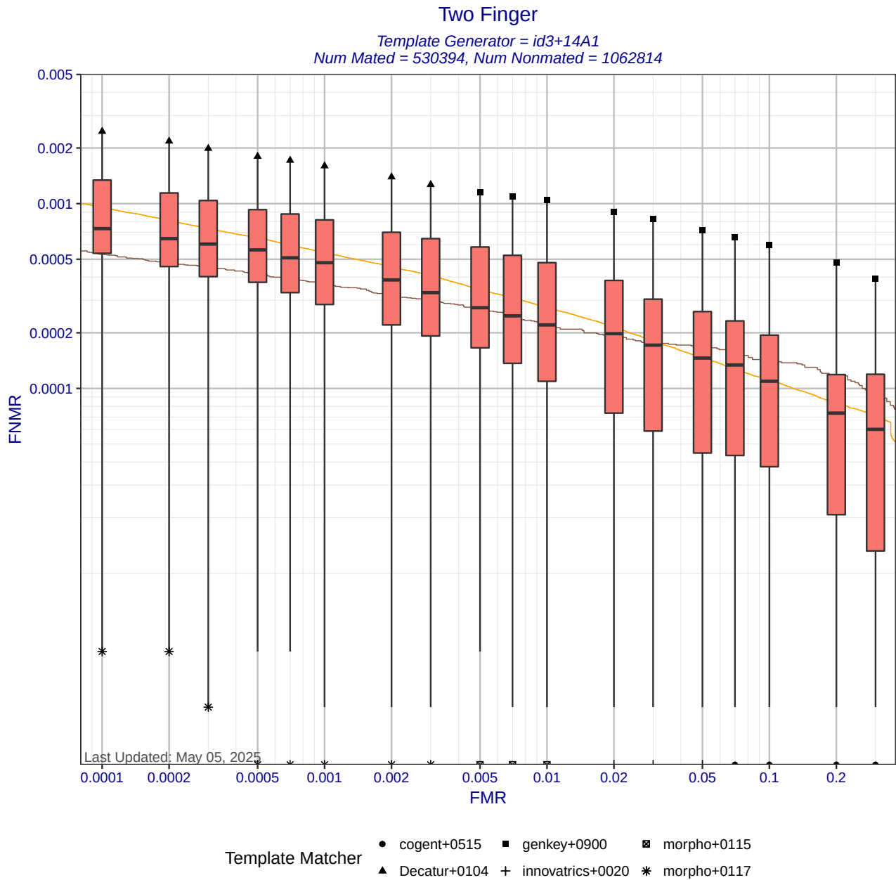
Figure 6: Two Finger DET statistics for template generator id3+14A1. Each box shows the distribution of FNRs at a fixed FMR across different matchers. The whisker ends show the minimum and maximum FNRs. The brown curve shows the DET curve when the matcher and template generators were submitted by the same participant. The orange DET curve shows pooled performance when all matchers use templates created by id3+14A1. Score-level fusion is achieved by averaging the scores for left and right index fingers.
