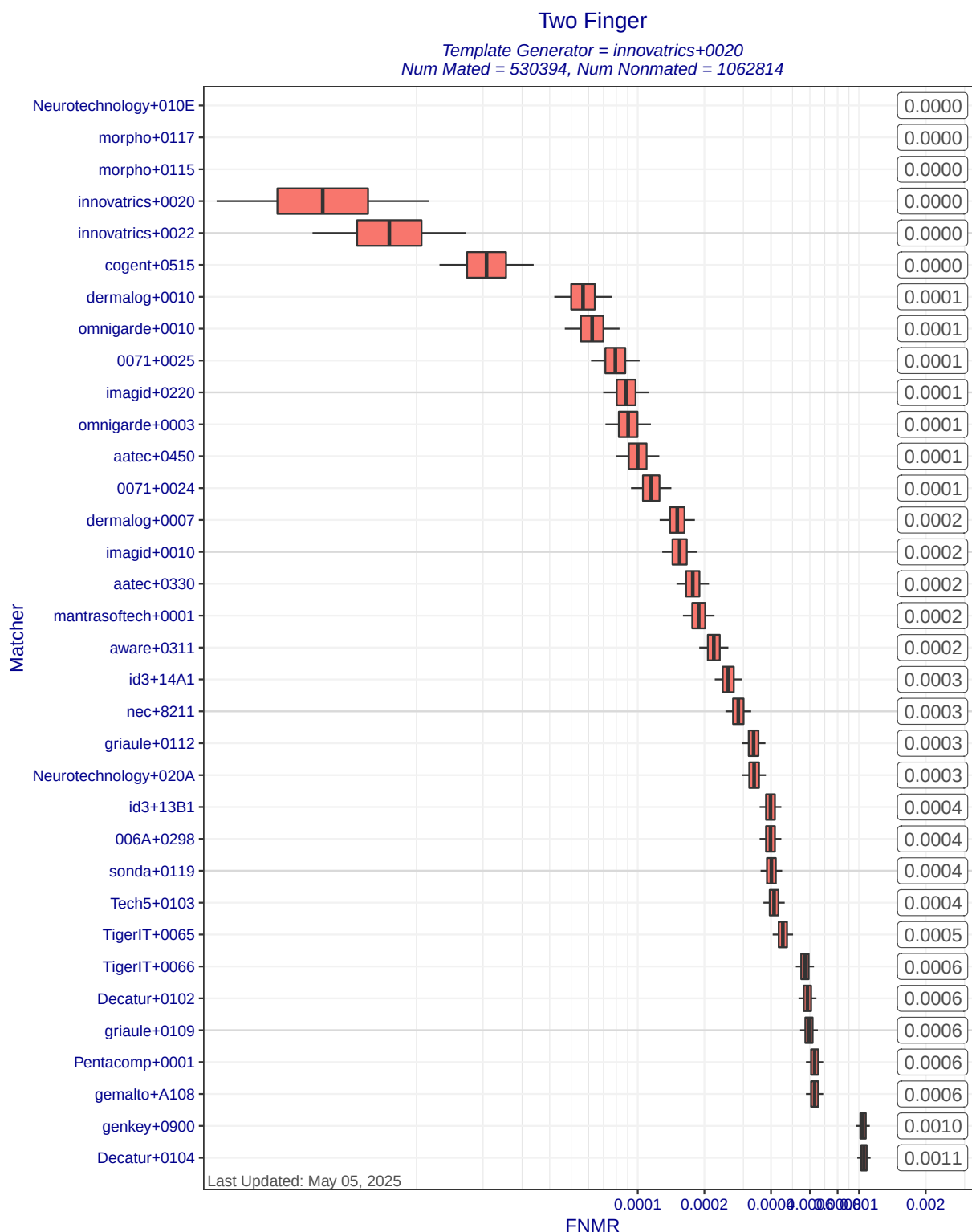
Figure 7: Two Finger FNMR at FMR=0.01 when different matchers compare templates created by template generator innovatrics+0020. Each box represents uncertainty about the true FNMR. The box edges mark the 50% confidence intervals while the whiskers mark the 90% confidence intervals. The numbers on the right show the actual computed FNMRs. Score-level fusion is achieved by averaging the scores for left and right index fingers.
