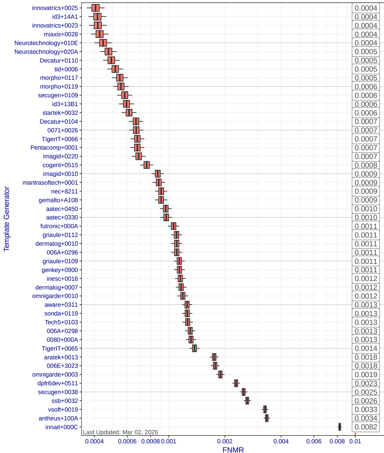
Figure 8: Two finger FNMR at FMR=0.01 when matcher Decatur+0110 compares templates created by different template generators. Each box represents uncertainty about the true FNMR. The box edges mark the 50% confidence intervals while the whiskers mark the 90% confidence intervals. The numbers on the right show the actual computed FNMRs. Score-level fusion is achieved by averaging the scores for left and right index fingers.
