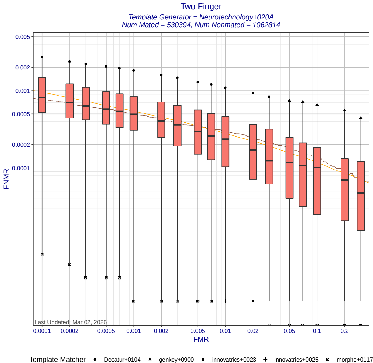
Figure 6: Two Finger DET statistics for template generator Neurotechnology+020A. Each box shows the distribution of FNMNRs at a fixed FMR across different matchers. The whisker ends show the minimum and maximum FNMNRs. The brown curve shows the DET curve when the matcher and template generators were submitted by the same participant. The orange DET curve shows pooled performance when all matchers use templates created by Neurotechnology+020A. Score-level fusion is achieved by averaging the scores for left and right index fingers.
