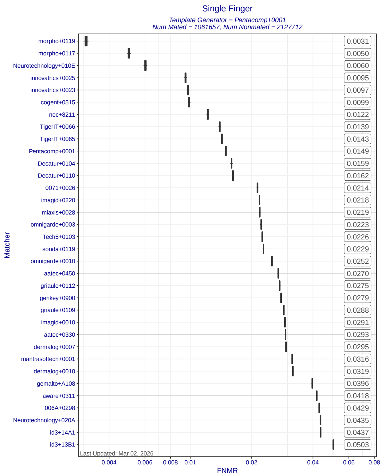
Figure 5: Single Finger FNMRS at FMR=0.0001 when MINEX III compliant matchers compare templates created by template generator Pentacomp+0001. Each box represents uncertainty about the true FNMRS. The box edges mark the 50% confidence intervals while the whiskers mark the 90% confidence intervals. The numbers on the right show the actual computed FNMRS.
