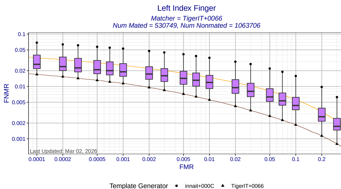
Figure 4: Left index finger DET statistics for matcher TigerIT+0066. Each box shows the distribution of FNMRs at a fixed FMR across all MINEX III compliant template generators. The ends of whiskers show the minimum and maximum FNMRs. The orange DET curve shows pooled performance against all template generators.
