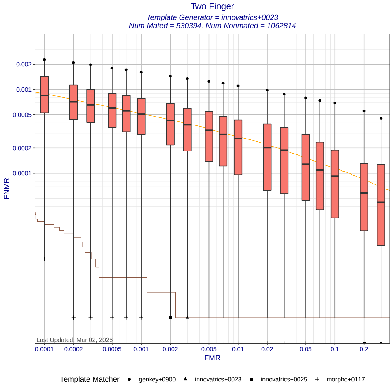
Figure 6: Two Finger DET statistics for template generator innovatrics+0023. Each box shows the distribution of FNMNRs at a fixed FMR across different matchers. The whisker ends show the minimum and maximum FNMNRs. The brown curve shows the DET curve when the matcher and template generators were submitted by the same participant. The orange DET curve shows pooled performance when all matchers use templates created by innovatrics+0023. Score-level fusion is achieved by averaging the scores for left and right index fingers.
