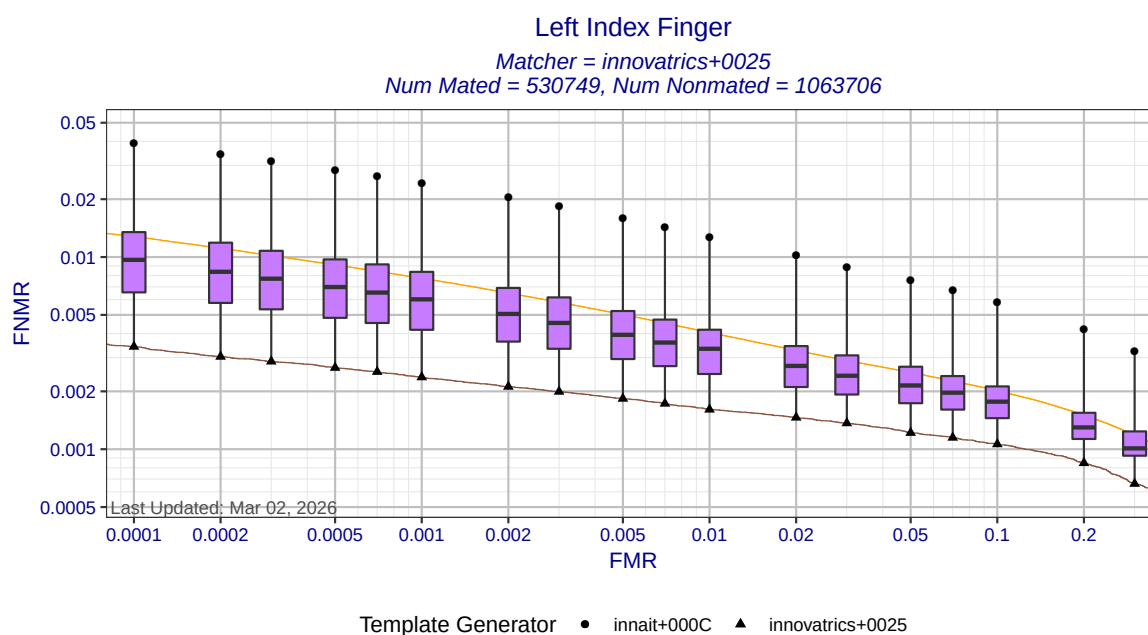
Figure 4: Left index finger DET statistics for matcher innovatrics+0025. Each box shows the distribution of FNMRs at a fixed FMR across all MINEX III compliant template generators. The ends of the whiskers show the minimum and maximum FNMRs. The orange DET curve shows pooled performance against all template generators.
