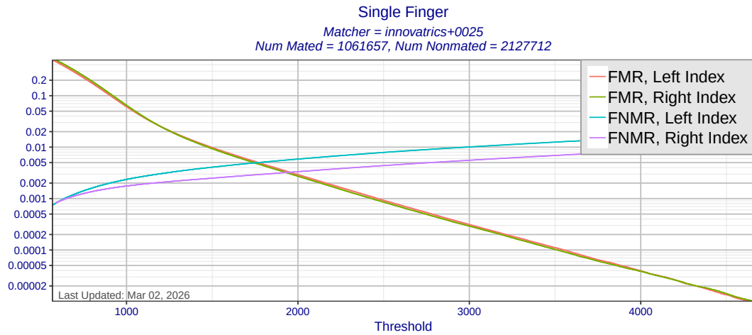
Figure 11: Single finger FMR and FNMR as a function of score threshold for matcher innovatrics+0025 using templates created by all MINEX III compliant template generators. Separate curves are presented for left and right index fingers.
