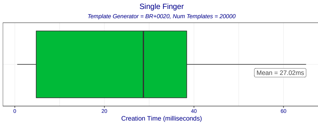
Figure 2: Boxplot of template creation times for template generator BR+0020. The box edges mark the 10th and 90th percentiles while the whiskers mark the maximum and minimum creation times.
