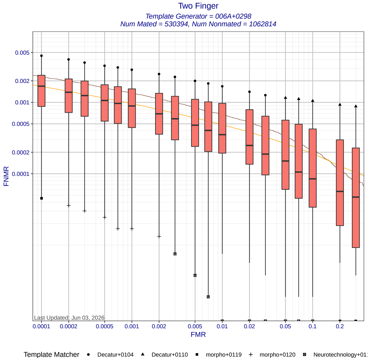
Figure 6: Two Finger DET statistics for template generator 006A+0298. Each box shows the distribution of FNMRs at a fixed FMR across different matchers. The whisker ends show the minimum and maximum FNMRs. The brown curve shows the DET curve when the matcher and template generators were submitted by the same participant. The orange DET curve shows pooled performance when all matchers use templates created by 006A+0298. Score-level fusion is achieved by averaging the scores for left and right index fingers.
